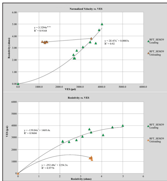
Figure 11. Cross-plots between resistivity and vertical effective stress. Upper figure plots the data following Bowers (1995). Lower figure re-plots the same data by switching axes to allow mathematical solvability.
