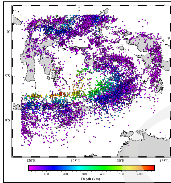
Figure 2. The high seismicity is showed by the hypocentres distribution around Banda Arc modified from (S. Das, 2004). Seismicity map using earthquake catalog ISC for period 1964–2000 with magnitude >3 (International Seismological Centre, 2022).
