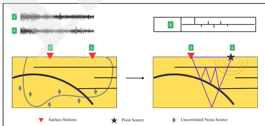
Figure 4. The illustration of Green's function interpretation in ANT modified from (R. Das & Rai, 2016). It connecting impulse relation between two stations represented in coda wave or noise. Then it stacked together to find the cross correlation in finding the initial velocity of surface wave.
