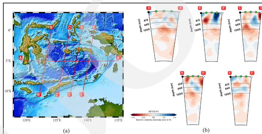
Figure 3. (a) Five cross sections around Banda Arc represented by a, b, c, d and e lines. (modified from (Spakman & Hall, 2010)). (b) P wave tomography result each cross section line using Tomography model Detox-P1 (Hosseini et al. , 2020), this tomography generate from SubMachine web-based tools for the interactive visualization (Hosseini et al. , 2018).
