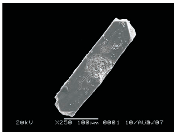
Figure 4. The basic shape of the phillipsite mineral before binding is monocline (Adisaputra and Hartono, 2007).
