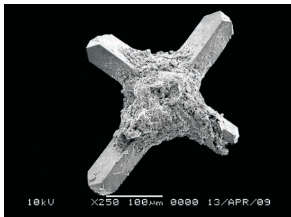
Figure 5. Phillipsite mineral bound by nannoplankton fossils forming cross shape.
