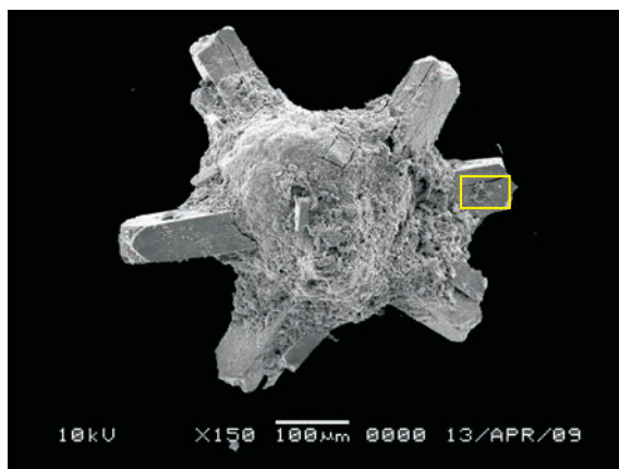
Figure 8. Phillipsite mineral in a radiar pattern magnification x150. The square indicates the position of Figure 7.
