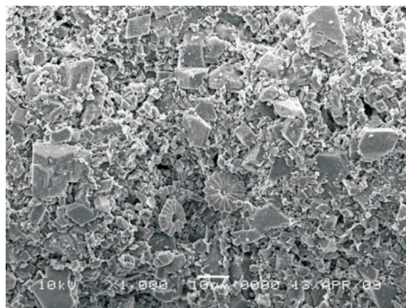
Figure 3. Sediments composed of calcite with Paleocene Discoaster multiradiatus fossils.
