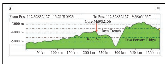
Figure 2. Cross section site of the studied area (Kusnida, 2009).
