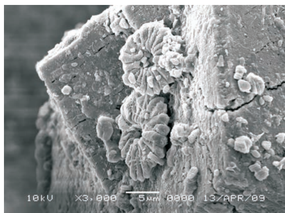
Figure 6. Discoaster multiradiatus fossils on the phillipsite mineral.
