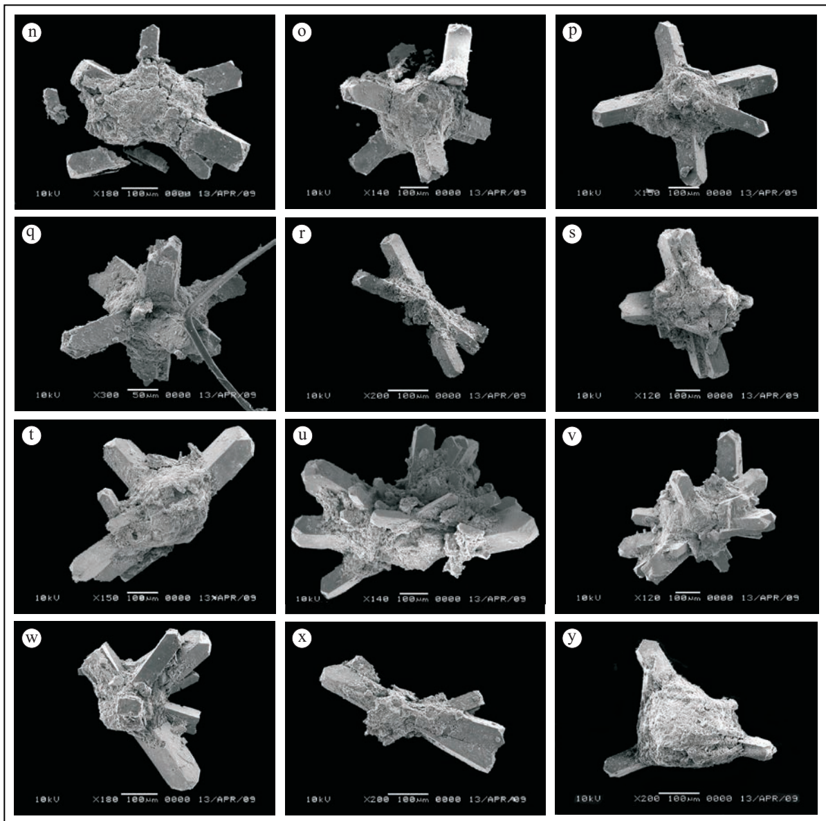
Figure 9. Continued ..... (n-q). radiate crystals, partly broken; (r-t). cruciform twinning, s and t partly broken with different angles; (u-x). rosette crystals; y. broken specimen.
