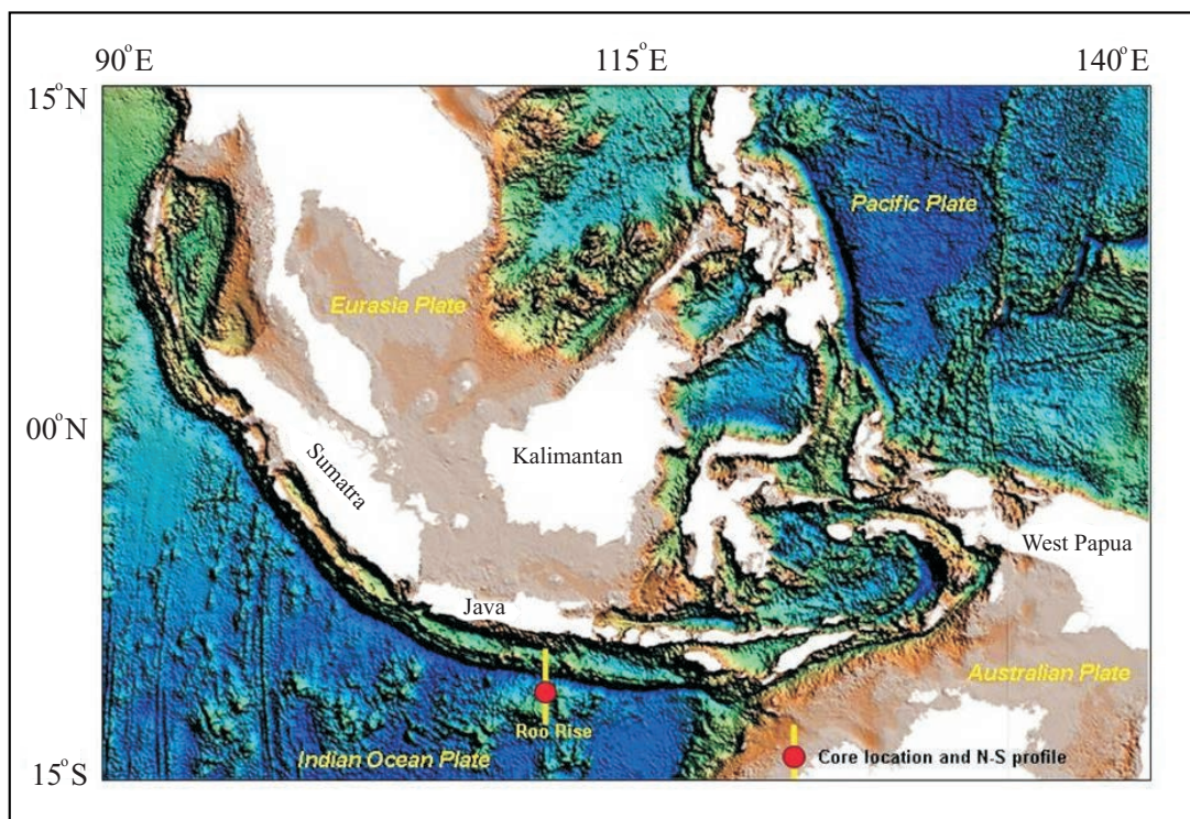
Figure 1. Locality map of the studied area (after Smith and Sandwell, 1997).
