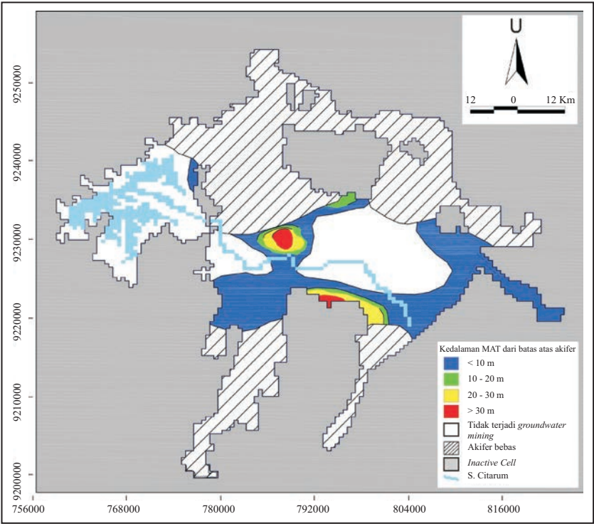
Gambar 11. Peta sebaran groundwater mining .
