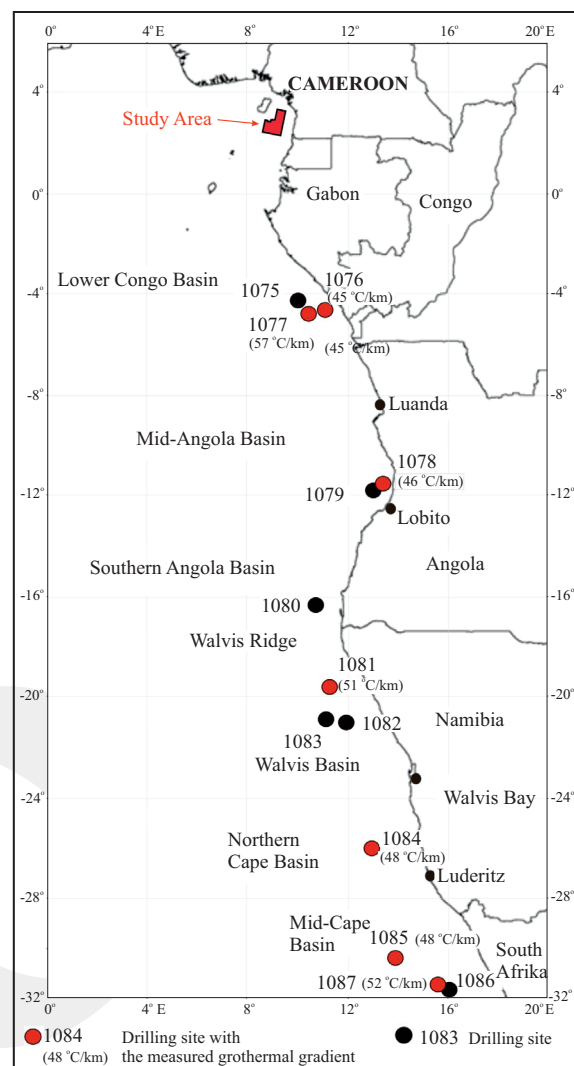
Figure. 1. Geothermal gradients estimated from Ocean Drilling Program (ODP Leg 175) data, using Adara tool to measure in-situ formation temperature in three points basic. Penetration depths are less than 600 mbsf, most of depths are less 200 m below seafloor (mbsf). Geothermal gradient ranges from 45 °C/km to 57 °C/km. The coastal line map is extracted from National Geophysical Data Centre (NGDC) ( http://rimmer.ngdc.noaa.gov/mgg/coast/getcoast.html ).
