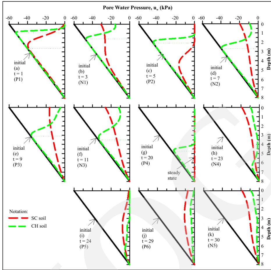
Figure 9. Pore water pressure profile at the major rainfall scenario for CH and SC soils type at the various time of precipitation.
