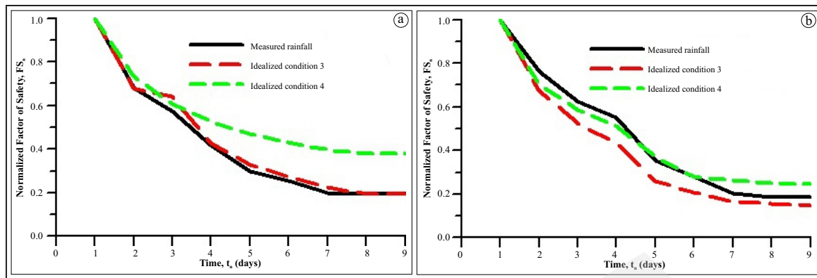
Figure 13. Normalized factor of safety with time due to rainfall scenarios, (a). SC slope; (b). CH slope.
