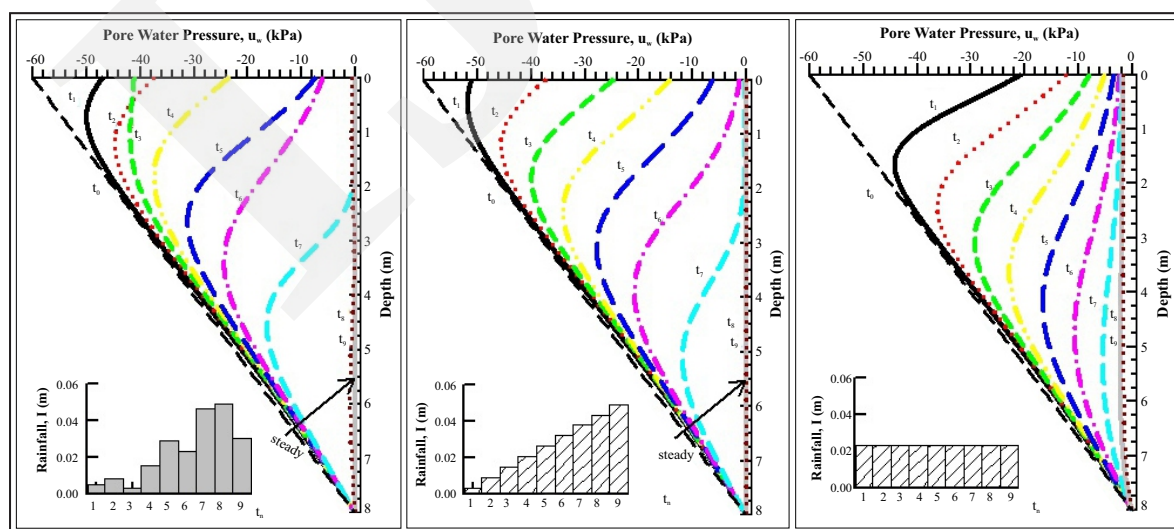
Figure 10. Distribution of pore water pressure in SC slope (a). measured rainfall; (b). idealized rainfall Condition 3; and (c). idealized rainfall Condition 4.
