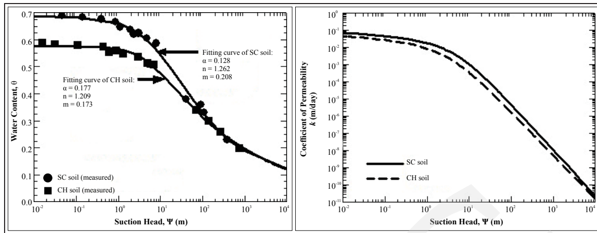
Figure 4. (a) Soil-water characteristic curve, (b) Hydraulic conductivity function of the soil.
