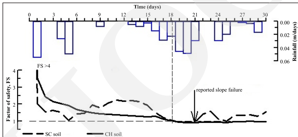
Figure 7. Variation of factor of safety due to Condition 1 rainfall scenarios.
