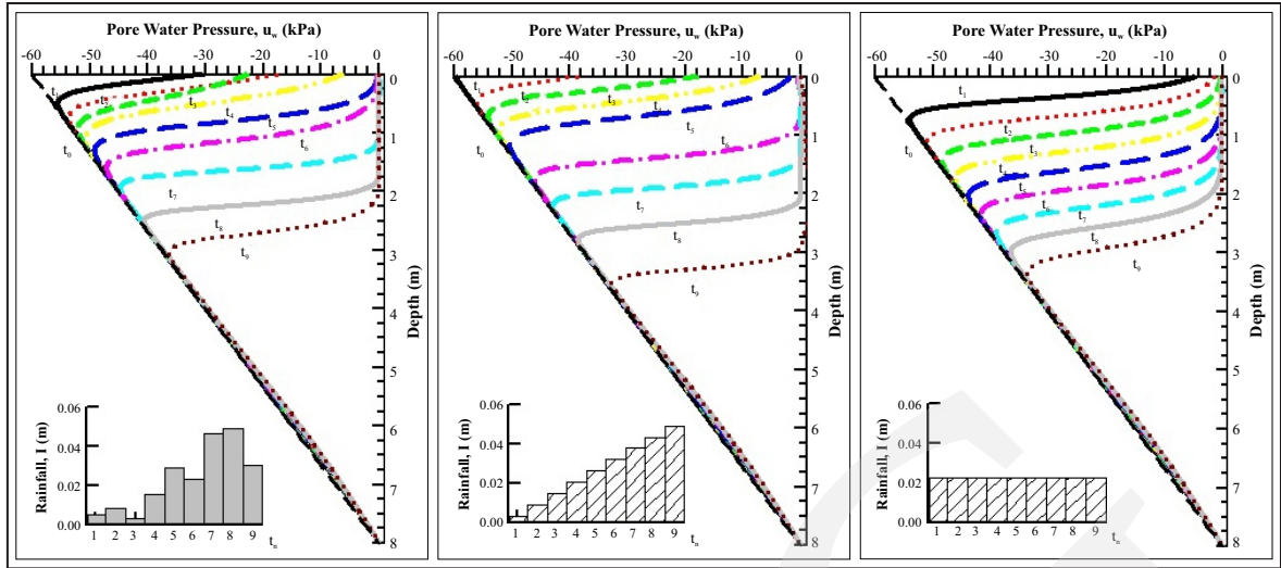
Figure 11. Distribution of pore water pressure in CH slope, (a). measured rainfall; (b). idealized rainfall Condition 3; and (c). idealized rainfall Condition 4.
