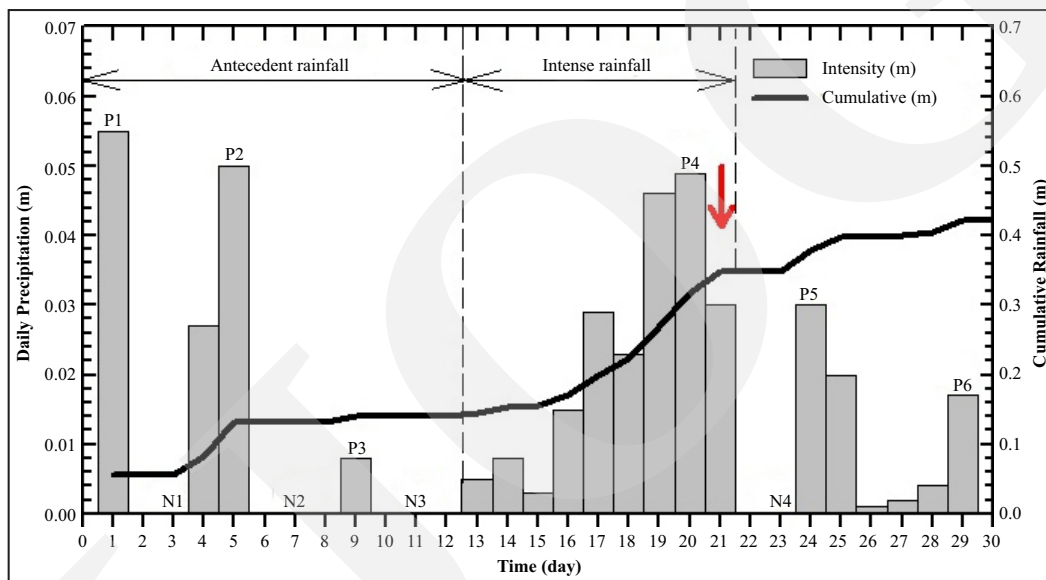
Figure 5. Daily rainfall hyetograph as the major rainfall in the back-analysis.
