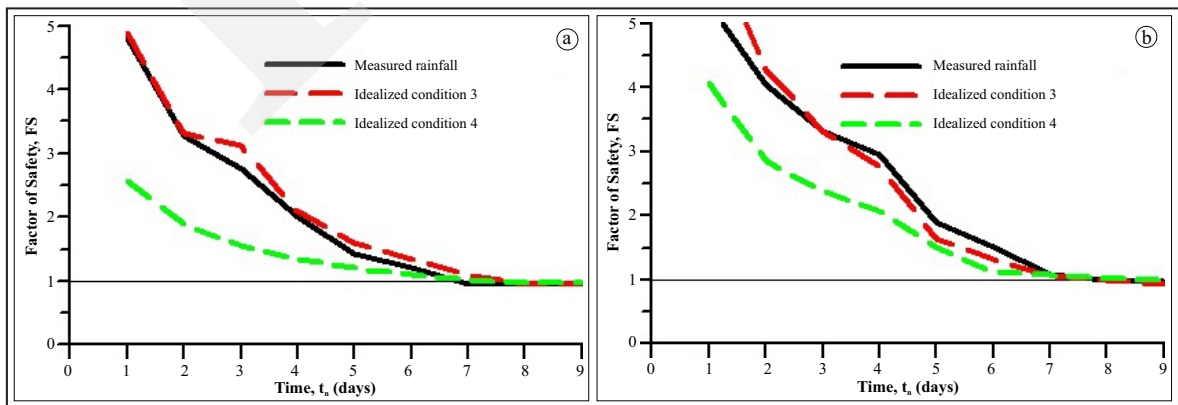
Figure 12. Variation of the factor of safety (FS) with time due to rainfall scenarios, (a). for SC slope; (b). for CH slope.
