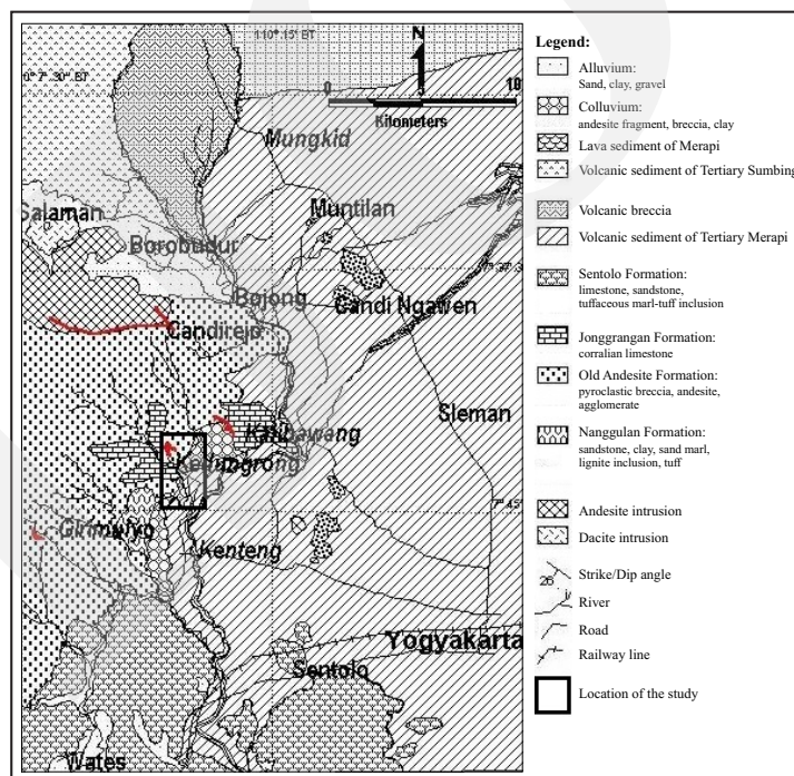
Figure 3. Geological condition of the Kedungrong and adjacent area.
