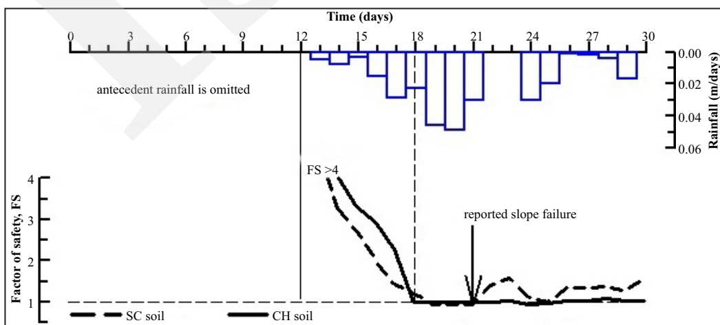
Figure 8. Variation of pore water pressure and factor of safety due to Condition 2 rainfall scenarios.
