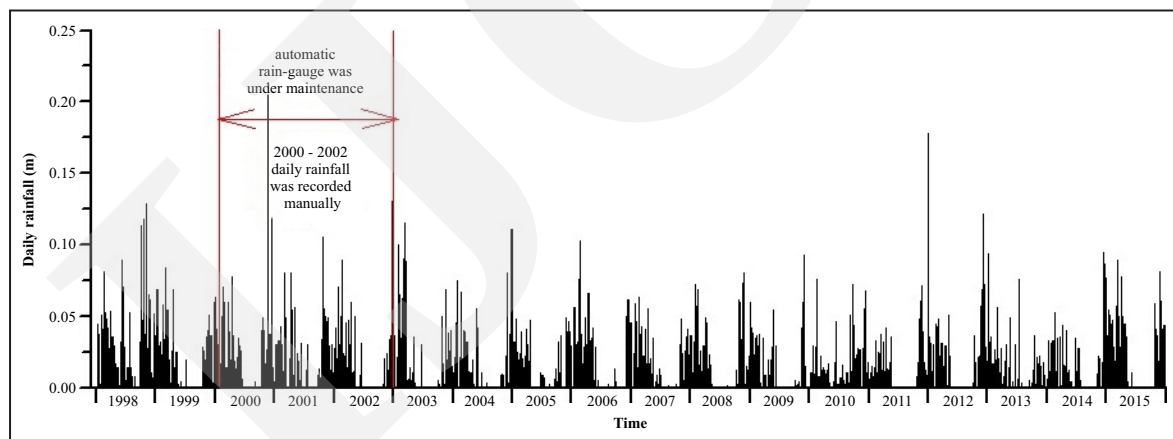
Figure 14. Precipitation distribution from January 1998 to December 2015 in Kalibawang rainfall station.
