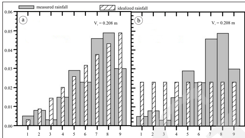
Figure 6. The second rainfall scenarios: (a) condition 3; delayed, (b) condition 4; average (or uniform).
