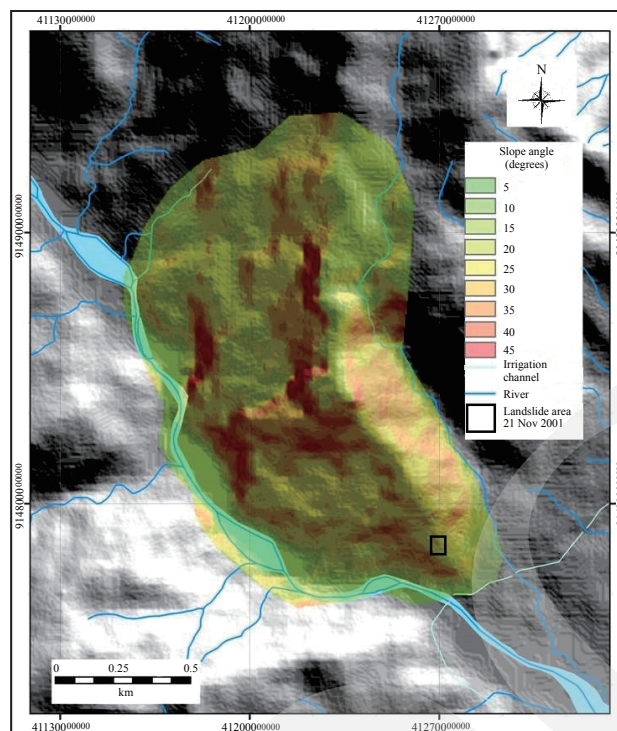
Figure 2. Distribution of slope inclination at the Kedungrong area.
