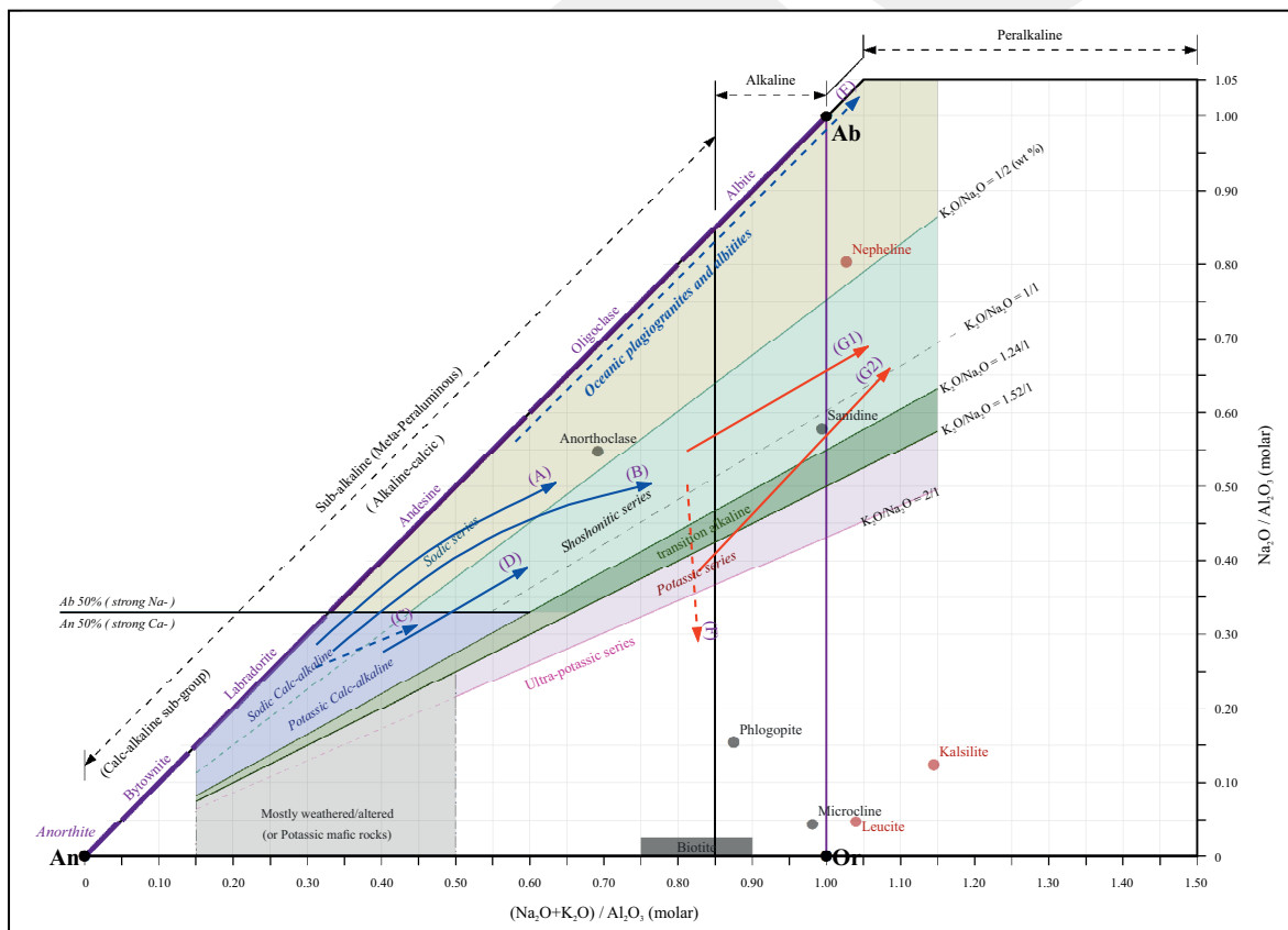
Figure 5. The cross-castic magma alkalinity evolution trend in Trapezoid model (Godang et al. , 2016). (A) Evolutionary trend of sodic calc-alkaline to sodic alkaline-calcic, (B) Sodic calc-alkaline to shoshonitic alkaline-calcic, (C) Blue dash-line shows the sodic calc-alkaline to potassic calc-alkaline, (D) Potassic calc-alkaline to shoshonitic alkaline-calcic, (E) Blue dash-line shows the evolution of oceanic plagiogranites/albitites from sodic alkaline-calcic to sodic alkaline/peralkaline. (F) Red dash-line shows the evolution of S-type granites from shoshonitic alkaline-calcic to potassic/ultrapotassic alkaline-calcic (cross-castic in sub-alkaline), (G1, G2) Evolution of A-type granites from shoshonitic/potassic alkaline-calcic to shoshonitic/potassic alkaline/peralkaline.
