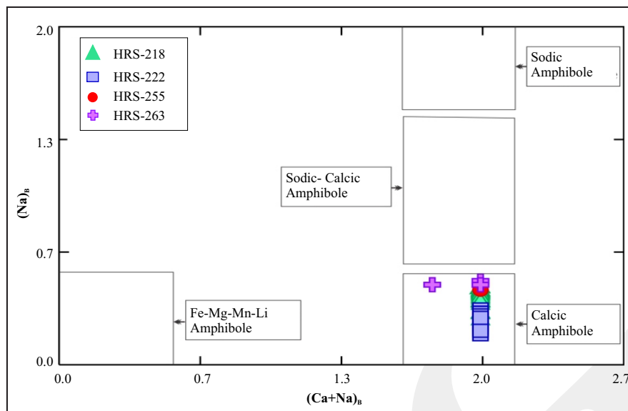
Figure 4. Plot of classification parameters on binary (Ca+Na)_B vs. (Na)_B diagram for amphibole group discrimination (Leake et al. , 1997). All analyzed amphiboles are calcic amphiboles.
