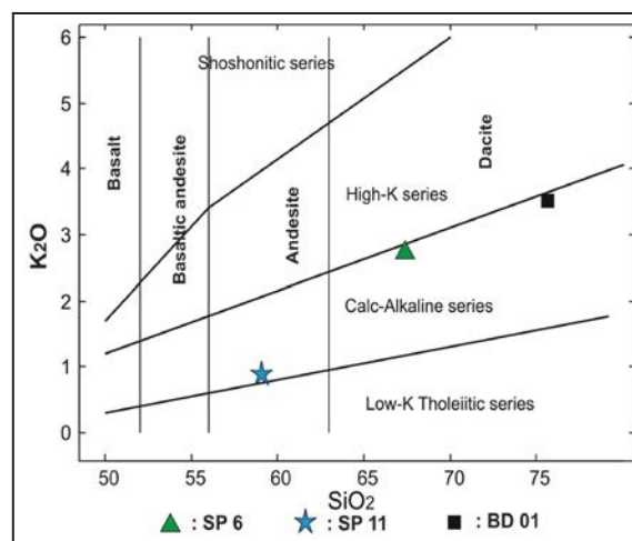
Figure 5. SiO 2 vs. K 2 O of the Cihara Granodiorite. The boundary between low-K tholeiite, calc-alkaline, high-K, and shoshonitic series are of Pecerillo and Taylor (1976).
