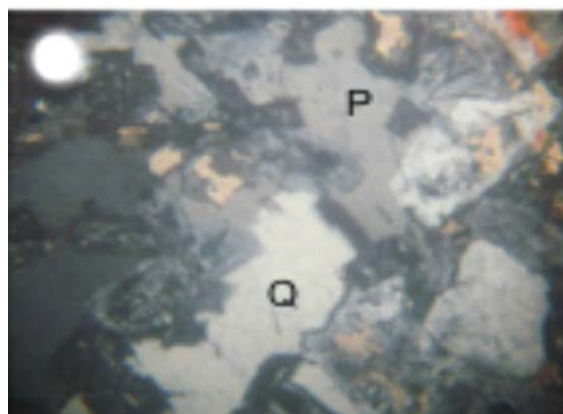
Figure 4. Plagioclase resorption (P) and quartz embayment (Q) in the Cihara Granodiorite.
