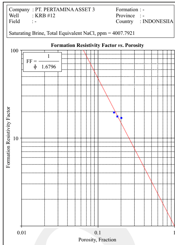
Figure 6. Plot of Porosity Formation Resistivity Factor to Acquire Value of a and m.
