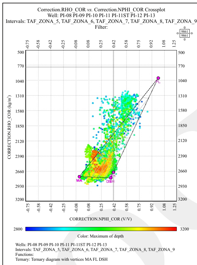
Figure 2. Density-Neutron crossplot Log In Marker 5-9.
