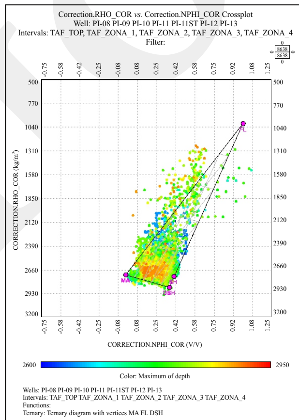
Figure 1. Density-Neutron Crossplot Log in Marker Top-4.
