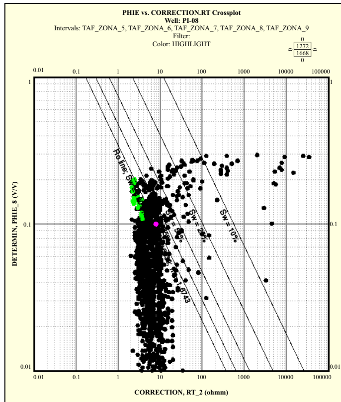
Figure 8. Determining R_w value using picket plot method.
