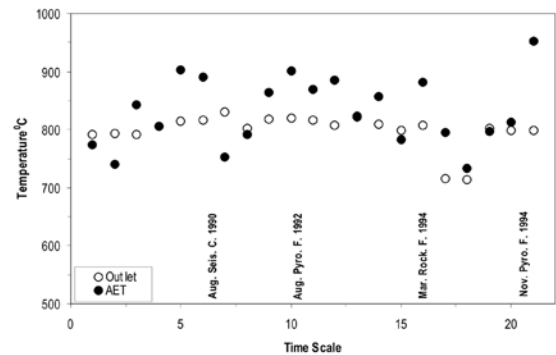
Figure 13. AET ( SO_2 + 3H_2 = H_2S + 2H_2O ) Gendol Merapi Volcano.
