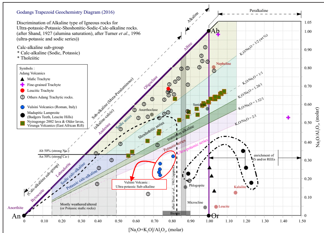
Figure 12. Plots in Godangs Trapezoid Geochemistry Diagram (Godang, 2016). The Vulsini Volcanics show the ultrapotassic subalkaline (alkaline-calcic character, alumina oversaturated; higher Al 2 O 3 contents), whereas Adang Volcanics and others Adang rocks show a contrast multimagmatic affinity (sodic series, shoshonitic, potassic, and ultrapotassic with alumina from oversaturated to undersaturated). Madupitic lamproite indicates ultrapotassic alkaline - peralkaline, whilst Virunga Volcanics are shoshonitic subalkaline - alkaline - peralkaline.
