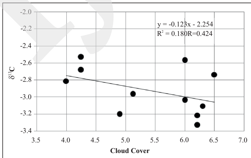
Figure 6. Linear regression of cloud cover and \delta^{13}\text{C} in the annual mean scale.
