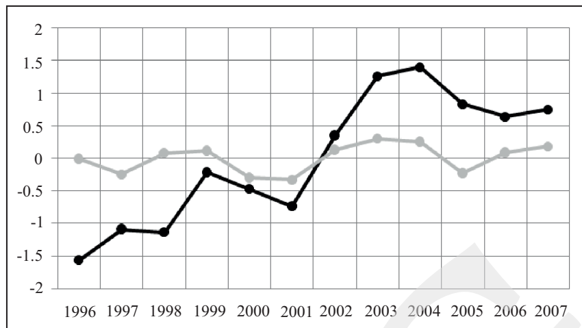
Figure 7. Annual mean variation of coral \delta^{13}\text{C} (dark line) and SST (grey line) derived from coral Sr/Ca. Data are standardized to unit variance.
