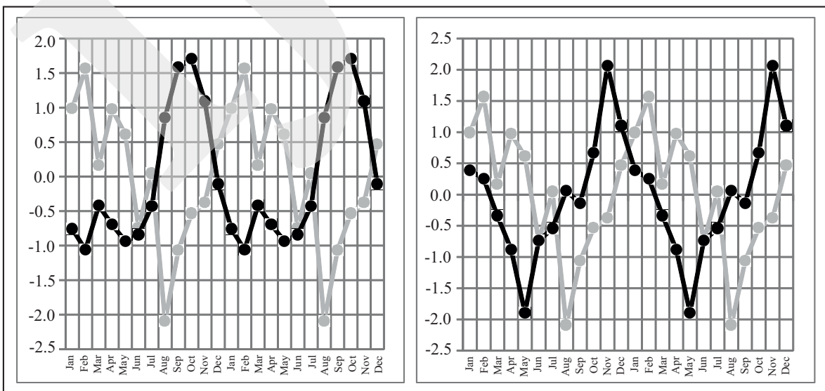
Figure 4. Graphic of monthly mean variation of solar radiation (grey line) and (left) cloud cover (dark line) and (right) \delta^{13}\text{C} (dark line). The data are corrected for two month lag. All time series data are standardized.
