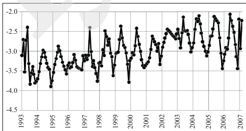
Figure 2. Monthly variation of \delta^{13}\text{C} content in Porites coral (sample code LB) from Labuhan Bajo.
