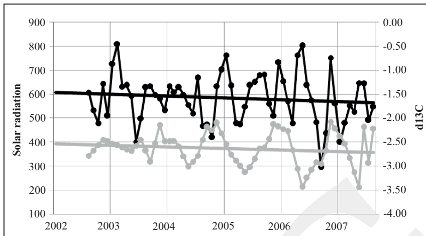
Figure 3. Graphic of monthly variation of coral \delta^{13}\text{C} (grey line) and solar radiation (dark line) and its trend lines (bold grey and dark lines).
