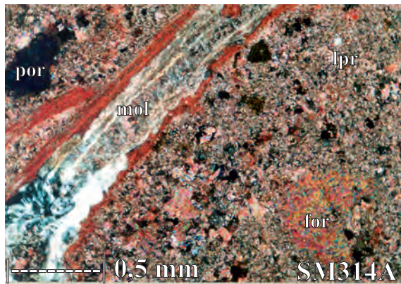
Figure 10. Photomicrograph of wackestone (sample code SM314A) with bioclasts of mollusks (mol) and large foraminifera (for) distributed in carbonate mud matrix (lpr) characterizing the SMF10-FZ7 on back-reef down-slope.
