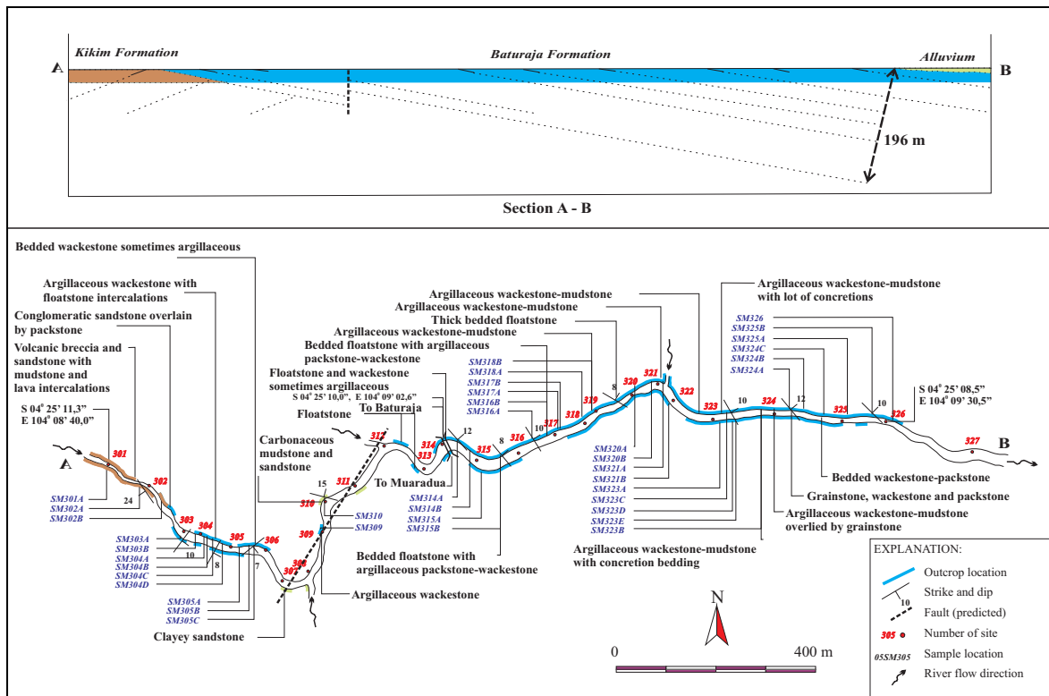
Figure 3. Detailed stratigraphic measured map along Air Rambangnia traverse (Maryanto, 2007a and 2008) and sample locations.
