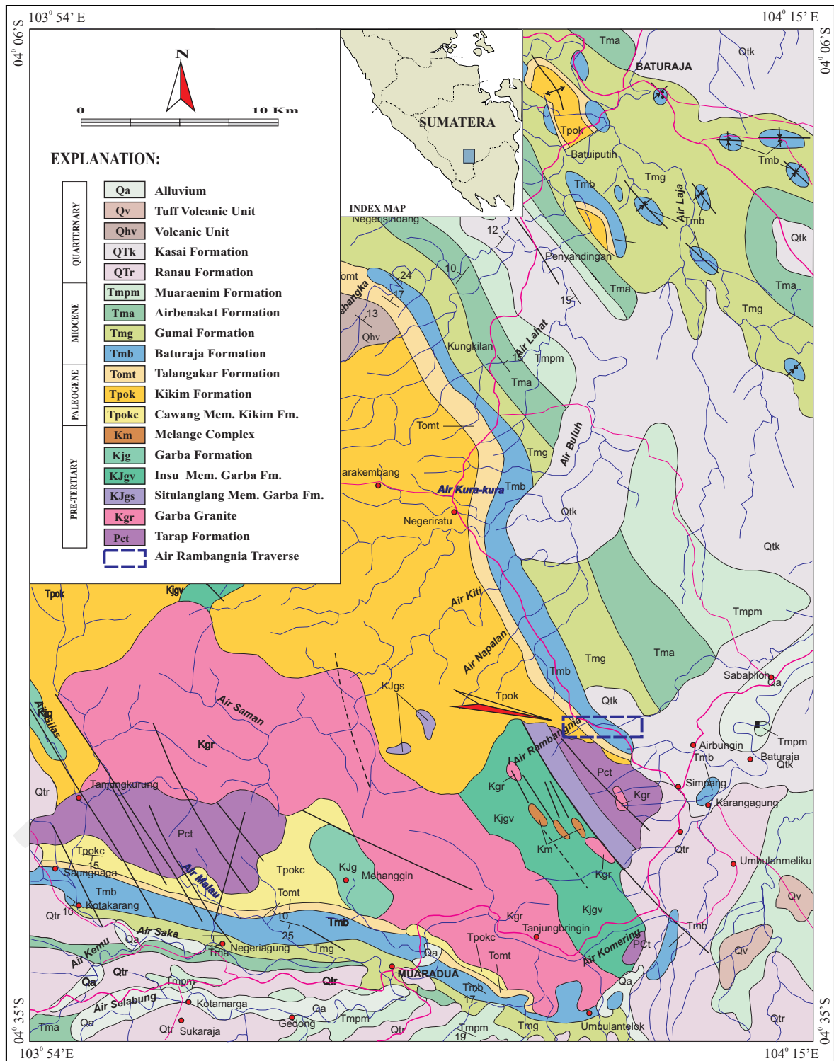
Figure 2. Geological map of Muaradua area, South Sumatra (Gafoer et al. , 1993) and locations of Air Rambangnia traverse (Maryanto, 2007a and 2008).
