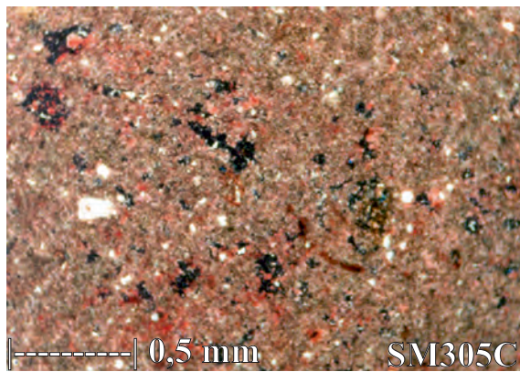
Figure 9. Photomicrograph of wackestone (sample code SM305C) with very fine-grained size, characterizing the SMF19-FZ8 on very restricted bay or pond.
