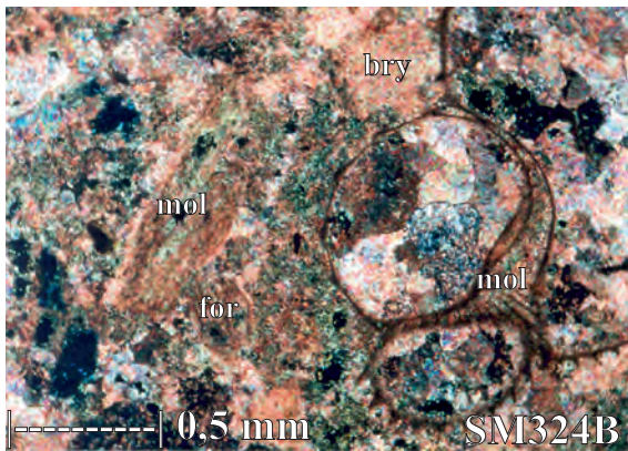
Figure 13. Photomicrograph of grainstone (sample code SM324B) with various bioclasts of mollusks (mol), large foraminifera (for), and bryozoans (bry) in carbonate cement, characterizing the SMF12-FZ6 on slope or shelf edge.
