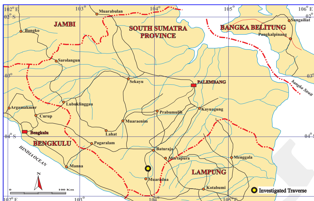
Figure 1. Location map of South Sumatra Province and the investigated traverse at Air Rambangnia River.
