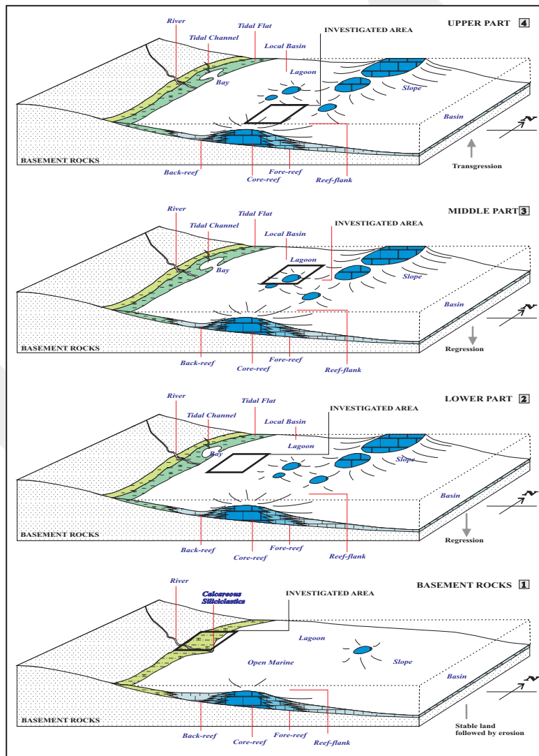
Figure 15. Depositional environment development of the Baturaja limestones along Air Rambangnia traverse, OKU Selatan, South Sumatra.
