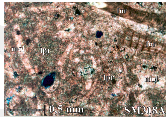
Figure 12. Photomicrograph of packstone (sample code SM318A) with various bioclasts of mollusks (mol) and large foraminifera (for) distributed in carbonate mud matrix (lpr), characterizing the SMF5-FZ4 on reef-flank area.
