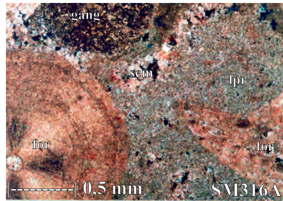
Figure 11. Photomicrograph of packstone/floatstone (sample code SM316A) with various bioclasts of red algae (gang) and large foraminifera (for) distributed in carbonate mud matrix (lpr), typifies the SMF5-FZ4 reef-flank area.
