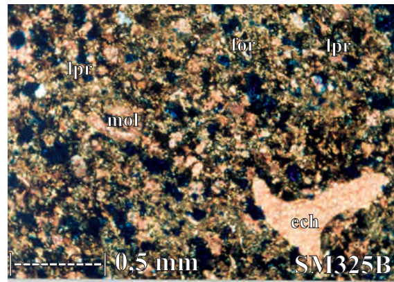
Figure 14. Photomicrograph of packstone (sample code SM325B) with abraded bioclasts of mollusks (mol), large foraminifera (for), and echinoderms (ech) distributed in carbonate mud matrix, characterizing the SMF10-FZ7 on the back-reef down-slope.
