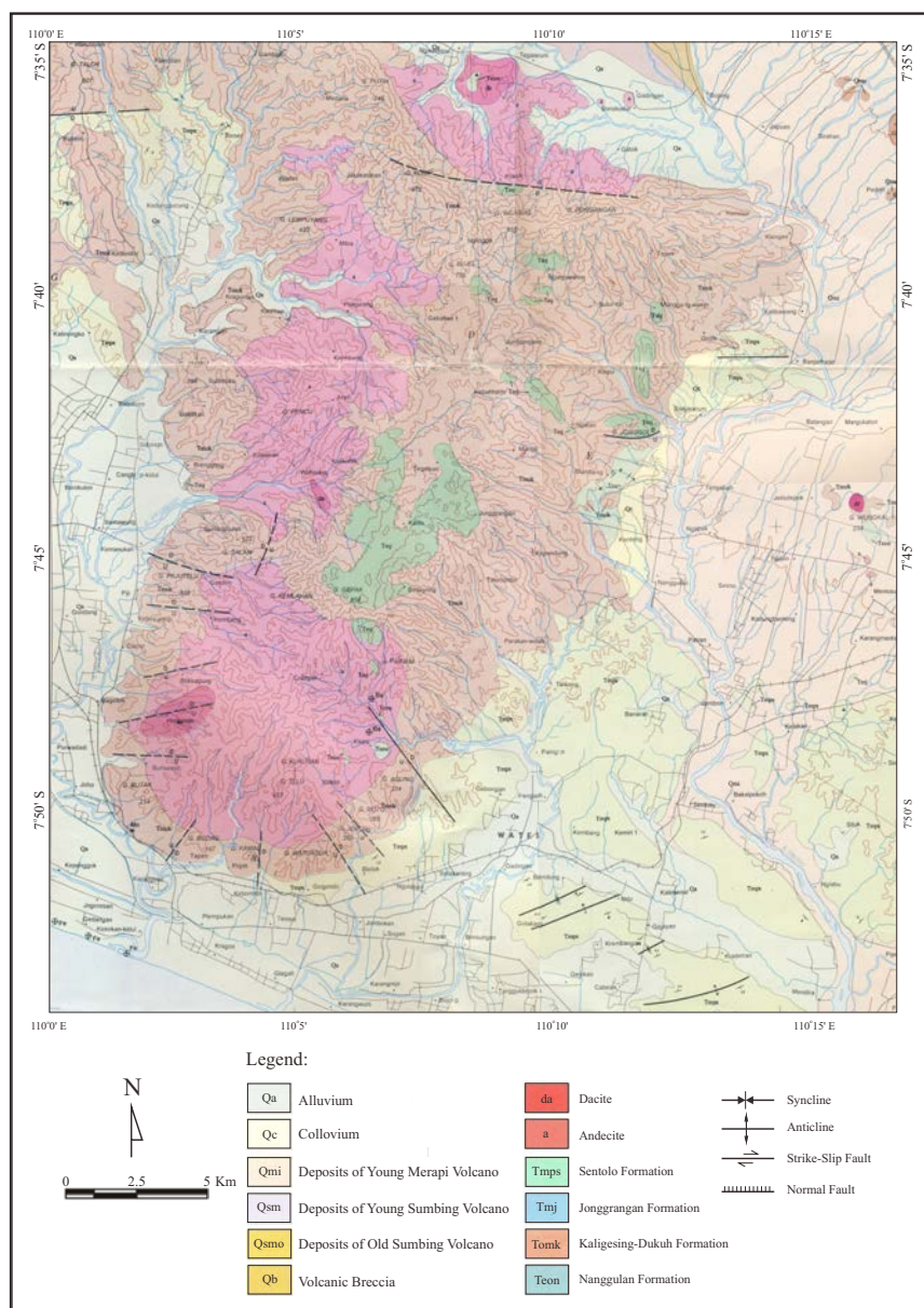
Figure 3. Geologic map of Kulon Progo Mountain, Yogyakarta (Rahardjo et al. , 1995).
