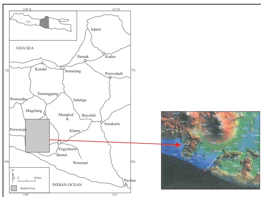
Figure 1. Map and satellite imagery show the location of the investigated area. A twin volcanoes Merapi and Merbabu are located at the center of northern part of the satellite imagery, whilst Kulon Progo Mountain is expressed in a rugged topography SW of those volcanoes or W of Yogyakarta City.
