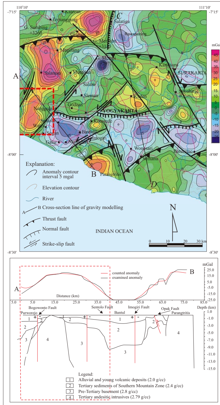
Figure 4. Bouguer - Residual anomalies modelling map of Kulon Progo Mountain and surrounding areas showing the base-ment configuration and lithology variation (Widiyanto, 2013).
