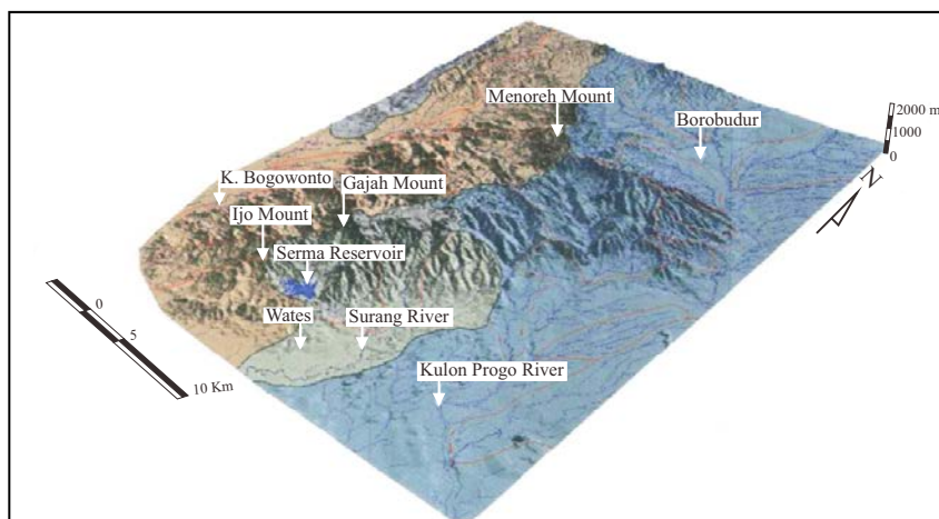
Figure 2. Bird view satellite imagery shows the morphologic configuration of Kulon Progo Mountain. An elongated shape of the mountain was one of the evidences of the tumor genesis suggested by van Bemmelen (1949). However the present investigation revealed that the regional tectonics operating in the area controlled the formation of Kulon Progo Mountain. Ijo and Gajah volcanic centers and important geographic names are indicated in this image (Note: different colors represent drainage basins).
