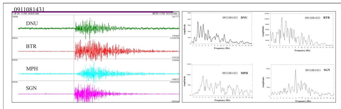
Figure 4. Seismogram and frequency dominant of VT earthquake recorded at four seismic stations (BTR, MPH, SGN, and DNU). This VT was recorded on November 8 th , 2009, at 14:31 WITA.
