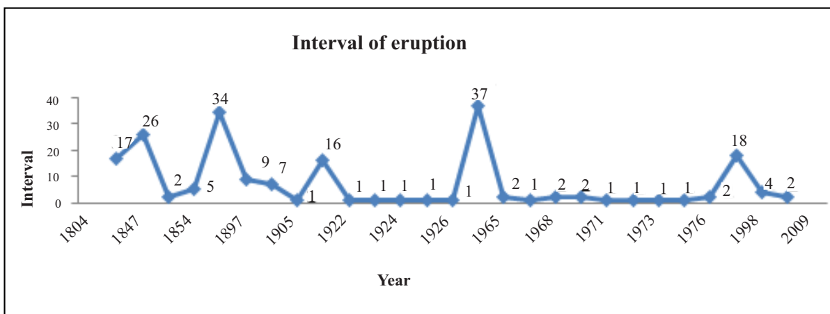
Figure 2. Eruption interval of Batur Volcano.
