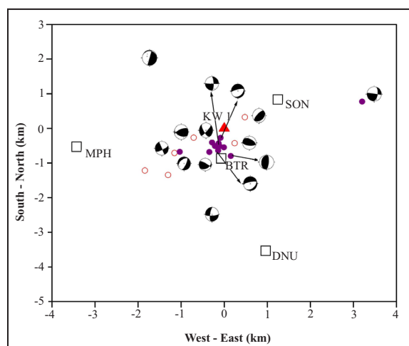
Figure 8. The result of focal mechanism of VT earthquakes. The red open circles, purple solid circles, open squares, and solid triangle represent hypocentre during September-October 2009, hypocentre during the swarm on November 2009, seismic station, and main crater, respectively.
