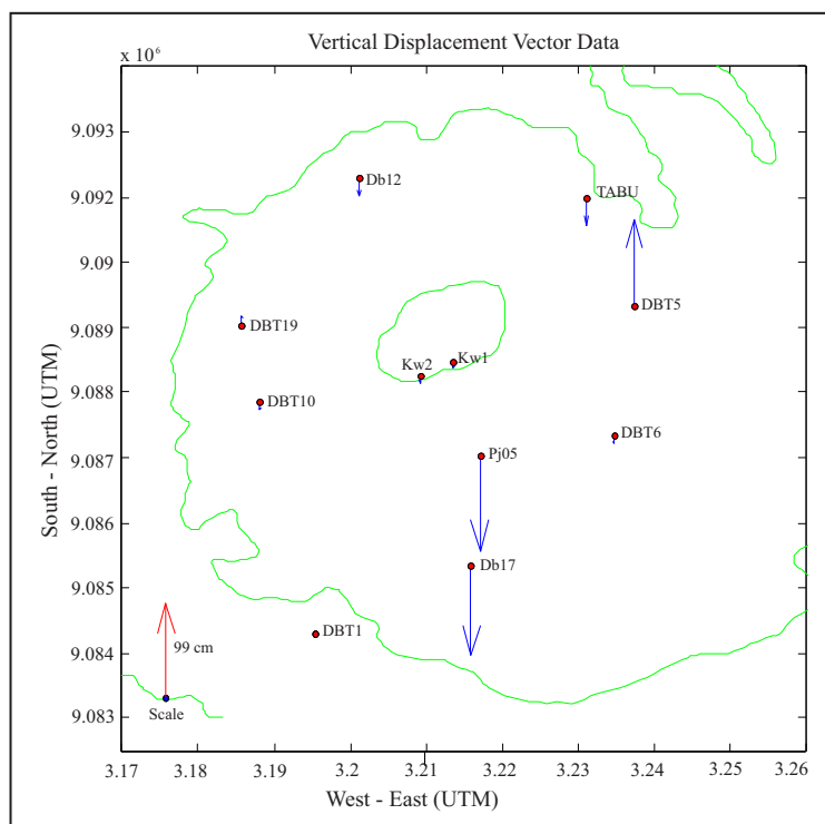
Figure 10. Vertical displacement November 2009 - October 2008.
