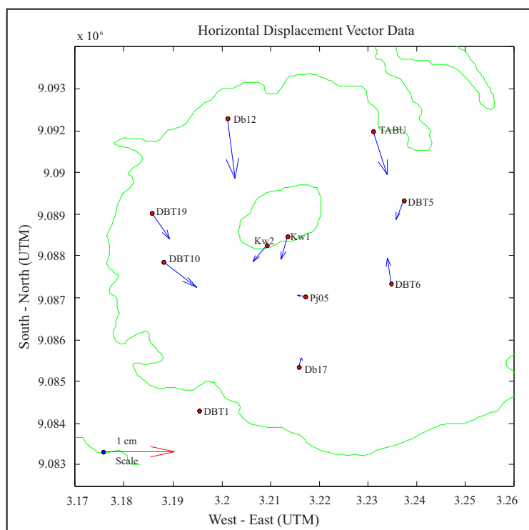
Figure 9. Horizontal displacement November 2009 - October 2008.
