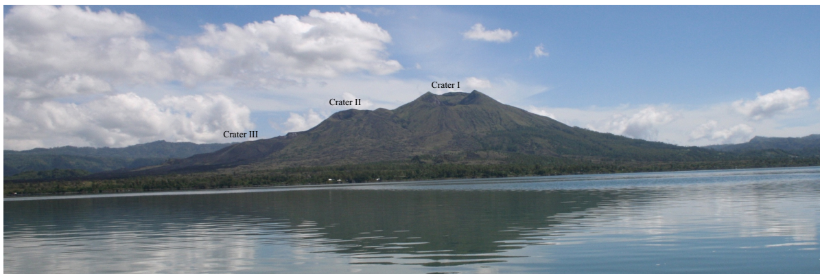
Figure 1. Batur Volcano and its craters (picture courtesy of Akhmad Solikhin, CVGHM).
