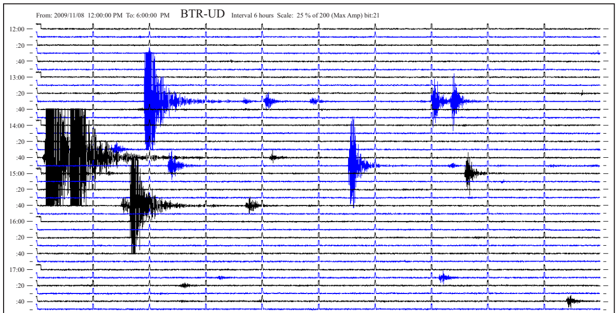
Figure 6. Seismogram of VT earthquakes during the swarm at 13:00 - 17:00 WITA (local time: GMT+8) on November 8 th , 2009.
