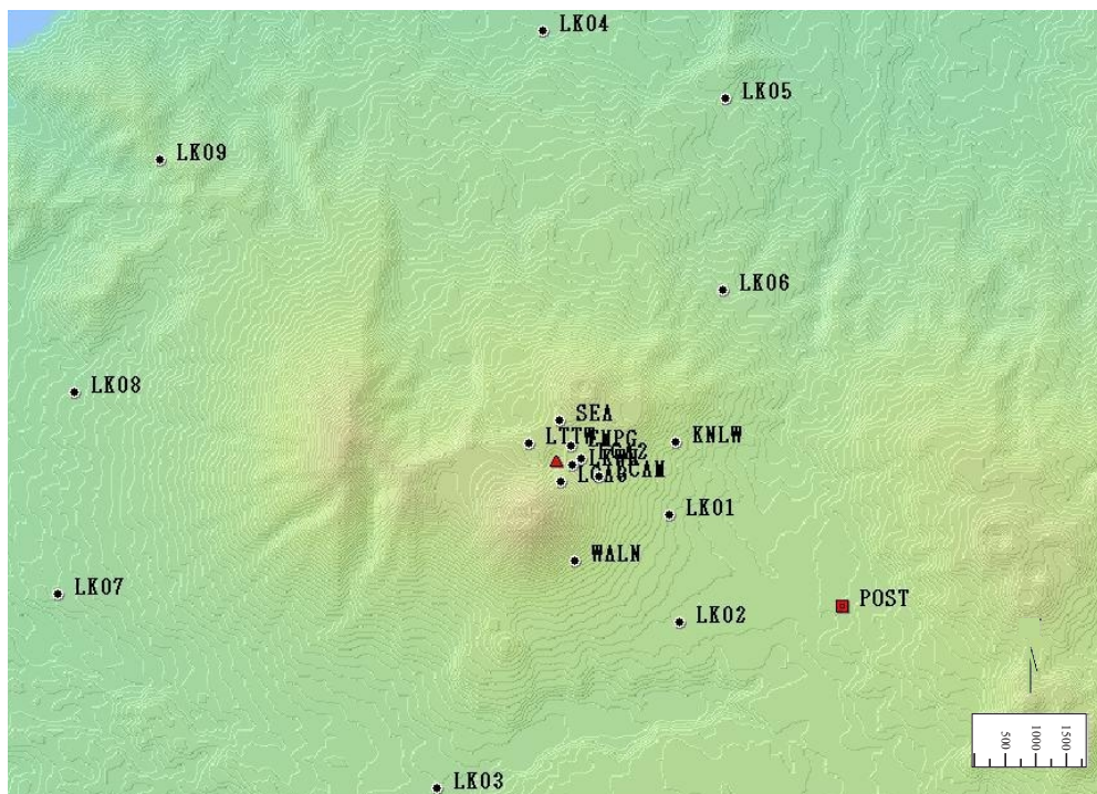
Figure 2. Distribution of GPS measuring points in the Lokon Volcano.
