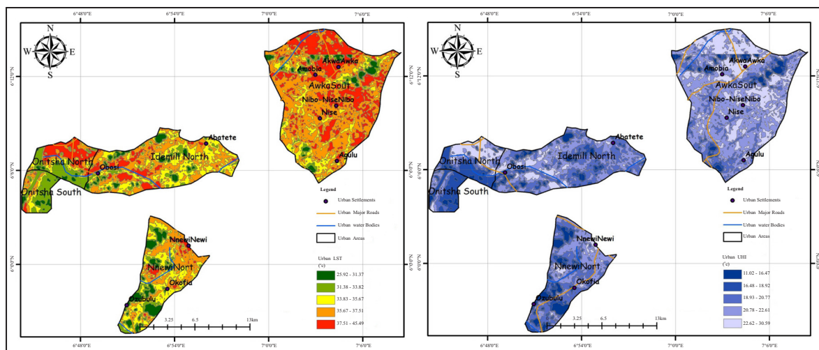
Figure 10. Urban LST and UHI patterns in Anambra State.
