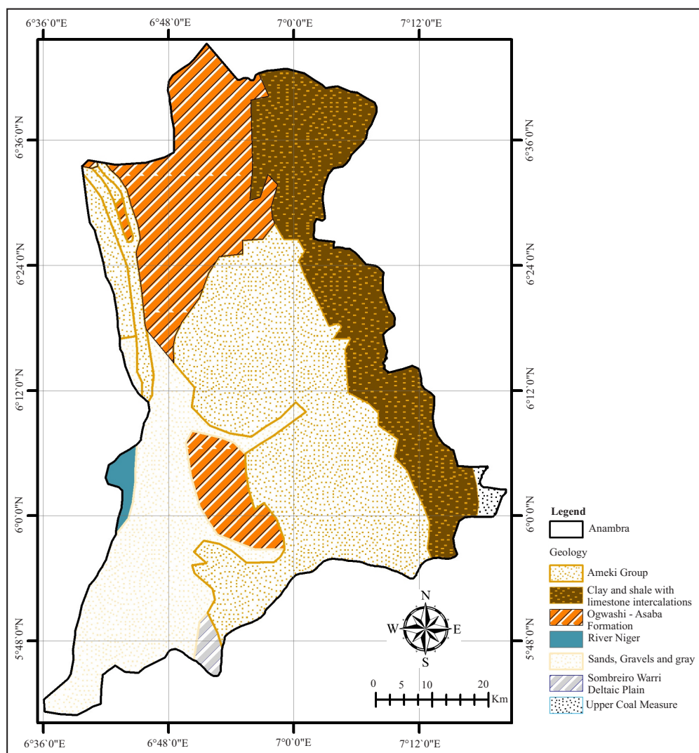
Figure 3. Geological formations of Anambra State and their spatial distribution.
