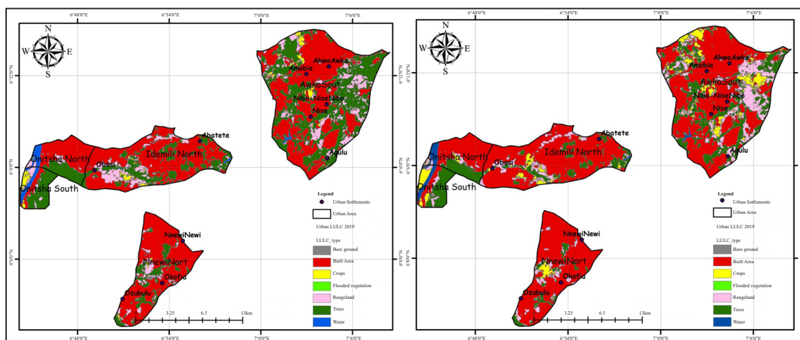
Figure 7. Comparison of Urban LULC Changes in Anambra State (a) 2019 and (b) 2024.
