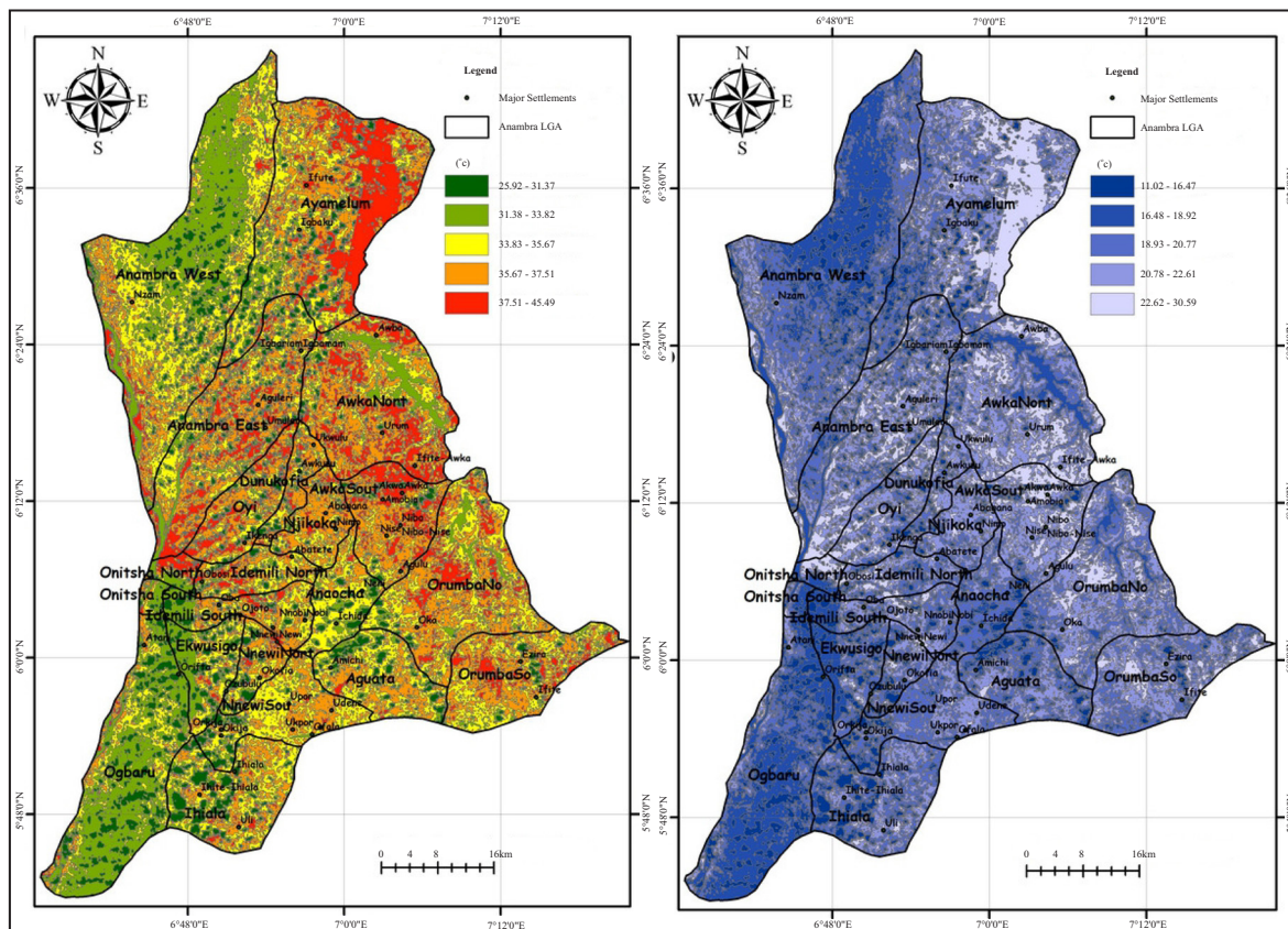
Figure 8. LST and UHI distribution in Anambra State.
