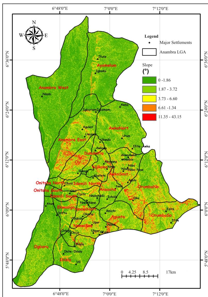
Figure 4. Slope analysis and its implications on land use in Anambra State.
