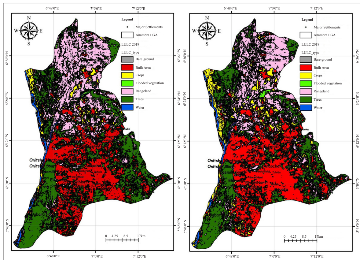
Figure 5. LULC Changes in Anambra State (a) 2019 and (b) 2024.
