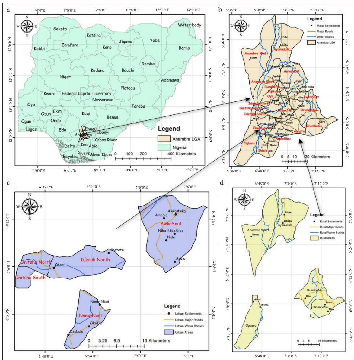
Figure 1. (a) Nigeria map, (b) Anambra State with LGAs, roads, and water bodies, (c) Urban areas with roads and water bodies, (d) Rural areas with roads and water bodies.
