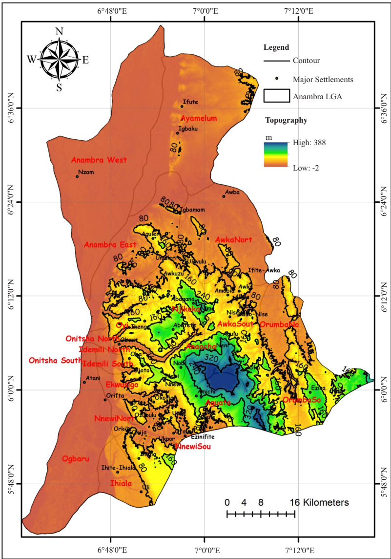
Figure 2. Topography of Anambra State, Nigeria.
