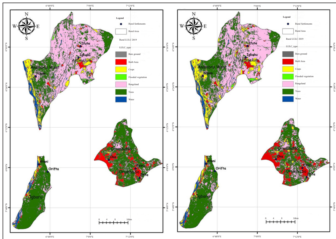
Figure 6. Comparison of Rural LULC Changes in Anambra State (a) 2019 and (b) 2024.
