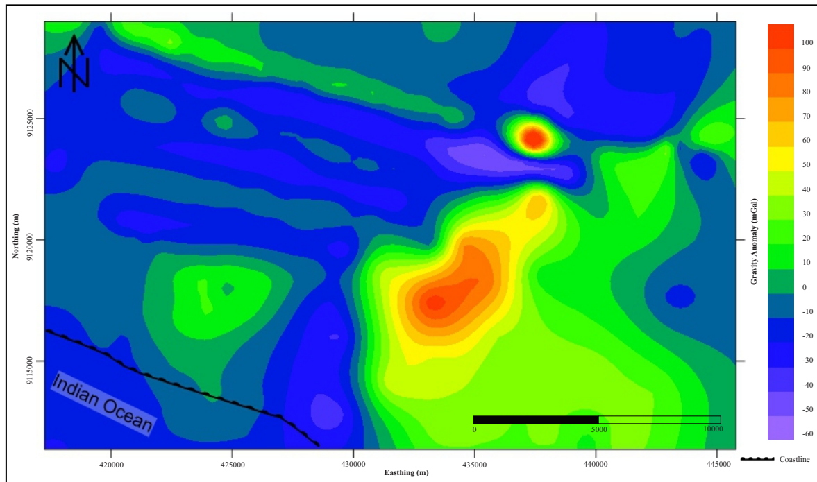
Figure 8. Residual anomaly, highlighting local and short-wavelength variations that are associated with shallow geological structures.
