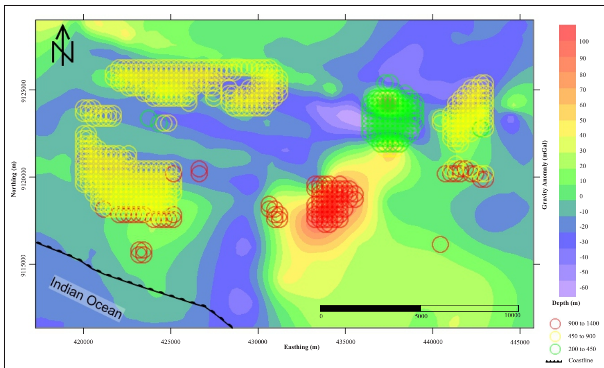
Figure 9. Gravity anomaly map of the studied area with Euler deconvolution solutions. The colour contour represents the gravity anomaly values (mgal), while the circles indicate estimated source depths: 200–450 m (green), 450–900 m (orange), and 900–1400 m (red).
