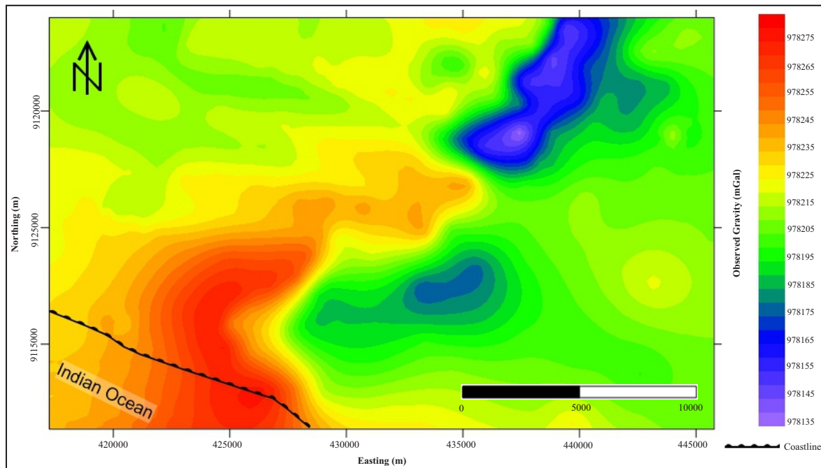
Figure 3. Observed gravity contour map obtained after tidal and drift corrections. The pattern is still strongly influenced by topography.
