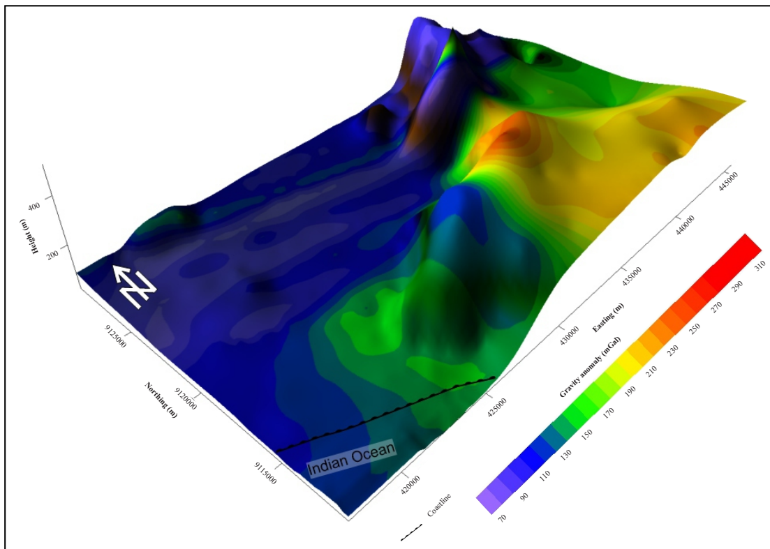
Figure 6. Three-dimensional topographic map overlaid with Complete Bouguer Anomaly (CBA) data of the studied area. The colour scale represents gravity anomaly values ranging from 70 to 310 mgal, where purple to blue indicates low anomalies and yellow to red indicates high anomalies.
