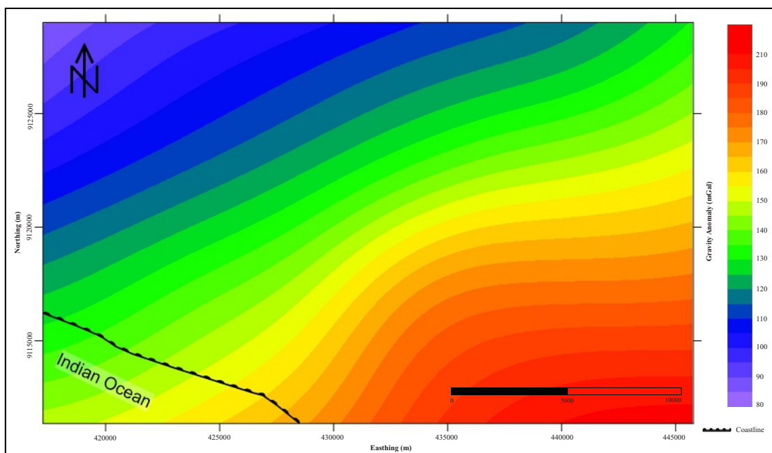
Figure 7. Regional anomaly, showing the broad and long-wavelength gravity trend.
