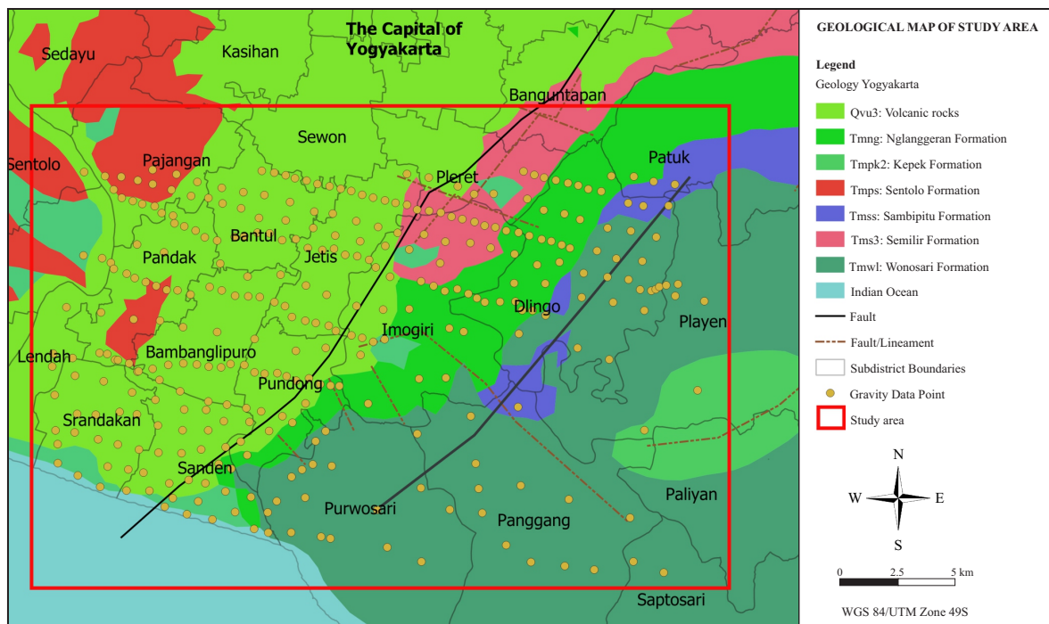
Figure 1. Geological map of the studied area (modified from Indonesia Geospatial Shapefile Map) The dashed lines indicate the presence of faults; the bold solid lines represent identified faults, the yellow circles represent the gravity data acquisition points, and the grey solid lines denote subdistrict boundaries.
