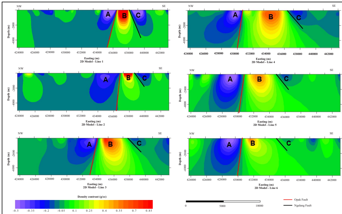
Figure 11. 2D inversion models of gravity data along six profiles (L1–L6) showing density contrast distribution ( \text{g}/\text{cm}^3 ). The colour scale represents density contrast values ranging from -0.5 \text{ g}/\text{cm}^3 (blue to purple, low density) to 0.85 \text{ g}/\text{cm}^3 (yellow to red, high density). Labels A, B, and C indicate the main density anomaly zones interpreted along each profile. The solid red lines represent the Opak Fault, while the solid black lines denote the Nglang Fault.
