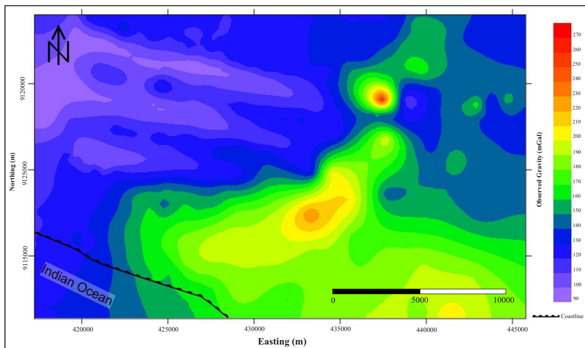
Figure 4. FAA contour map generated after applying free air correction to the observed gravity data.
