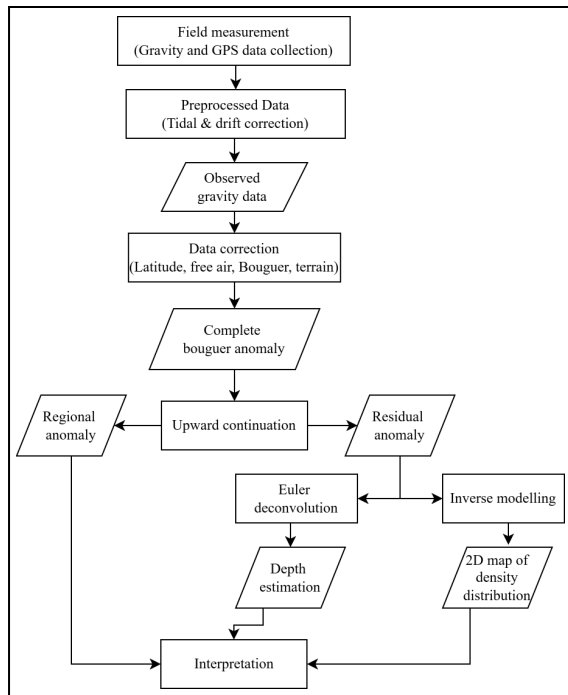
Figure 2. Data processing workflow showing the steps of data processing. This process involves data collection and interpretation to develop the subsurface structural and depth model.
