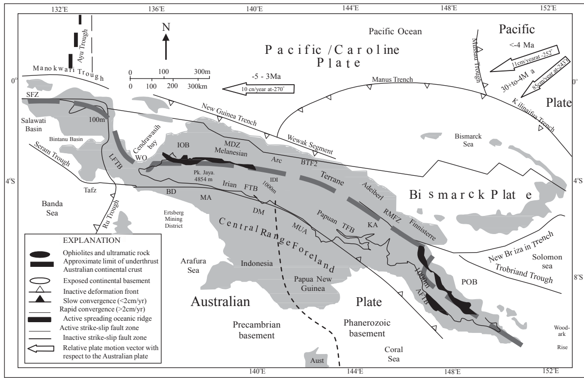
Figure 2. Regional tectonics of Papua and its vicinity (Sapiie et.al 1999).
