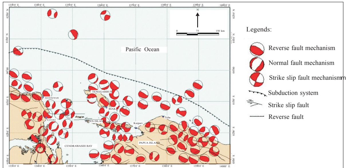
Figure 3. Seismotectonic map of Biak Island and its vicinity (Harvard CMT Catalog, 2010).
