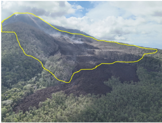
Figure 2. Image of the 10 th November 2024 eruption, lava flow (black colour) of Lewotobi Laki-laki in the west flank resulting from the eruption activity on 10 th November 2024. The burnt plants and the smoky areas because of eruption on 20 th March 2025 (yellow line). The image was taken using the Mavic 3T drone.
