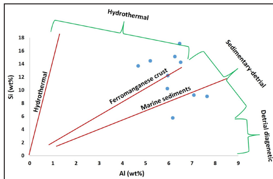
Figure 7. The position of ore samples from the studied region on the Si-Al diagram (adapted from Crerar et al. , 1982).
