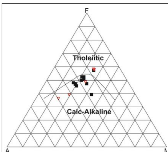
Figure 10. A (\text{K}_2\text{O} + \text{Na}_2\text{O}) - \text{F} - (\text{Fe}_2\text{O}_3) - \text{M} (\text{MgO}) diagram (after Irvine and Bragar, 1971). Symbols as in Figure 9.
