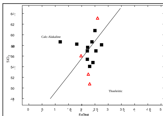
Figure 11. Diagram of \text{SiO}_2 versus \text{FeO total} / \text{MgO} of the lava from Sibayak - Sipiso-piso (after Myasiro 1974). Symbols as in Figure 9.
