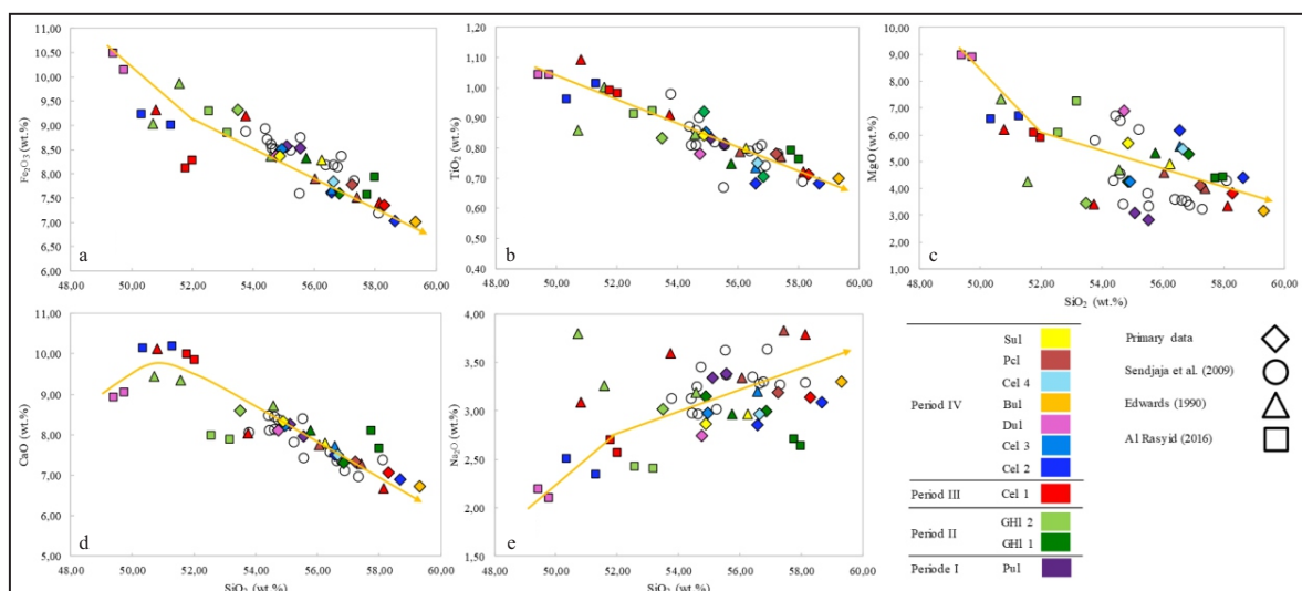
Figure 6. Harker variation diagram of (a) \text{Fe}_2\text{O}_3 , (b) \text{TiO}_2 , (c) \text{MgO} , (d) \text{CaO} , and (e) \text{Na}_2\text{O} , against the differentiation index of \text{SiO}_2 .
