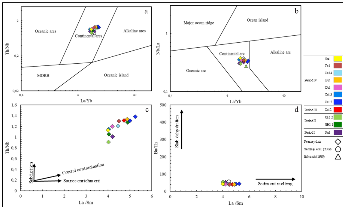
Figure 8. Tectonic discriminant diagrams, (a) Th/Nb vs. La/Yb, (b) Nb/La vs. La/Yb (Hollocher et al. , 2012), (c) Th/Nb vs. La/Sm (Plank, 2005 in Barresi et al. , 2015) and (d) Ba/Th vs. La/Sm (Labanieh et al. , 2012).
