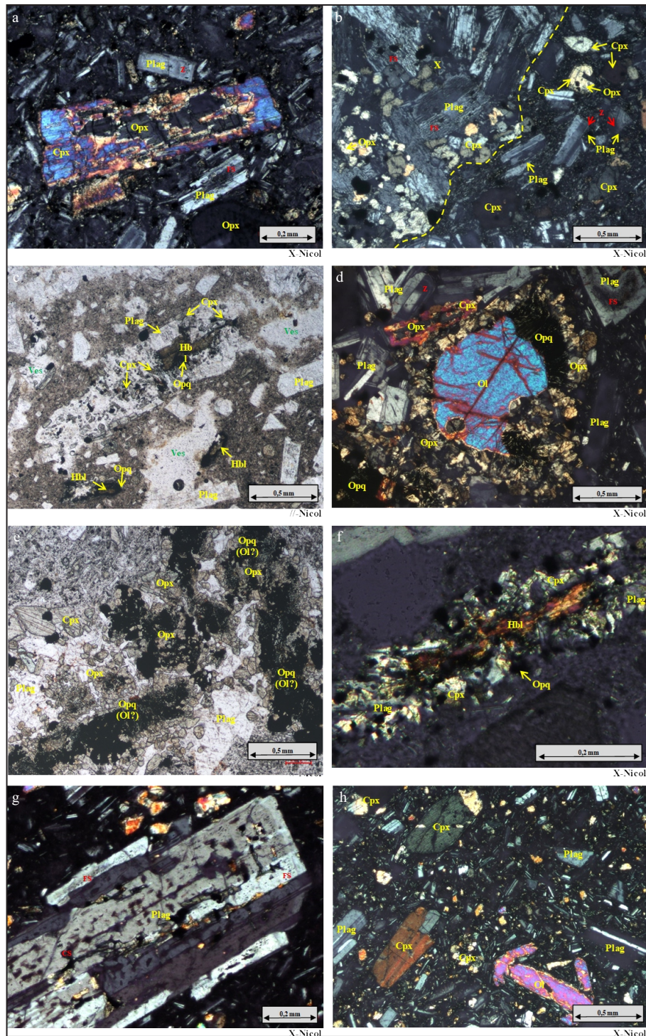
Figure 4. Photomicrographs of the volcanic rocks from the CVC, showcasing distinctive microtextures. (a) Orthopyroxene rimmed by clinopyroxene in Pul, (b) xenolith of microgabbro in GH1, (c) hornblende with a disequilibrium texture in GH2, (d) olivine antecrysts in Cel 1, (e) traces of olivine antecrysts in Cel 2, (f) hornblende with a disequilibrium texture in Bul, (g) coarse-sieved plagioclase in Pcl, and (h) skeletal olivine in Sul.
