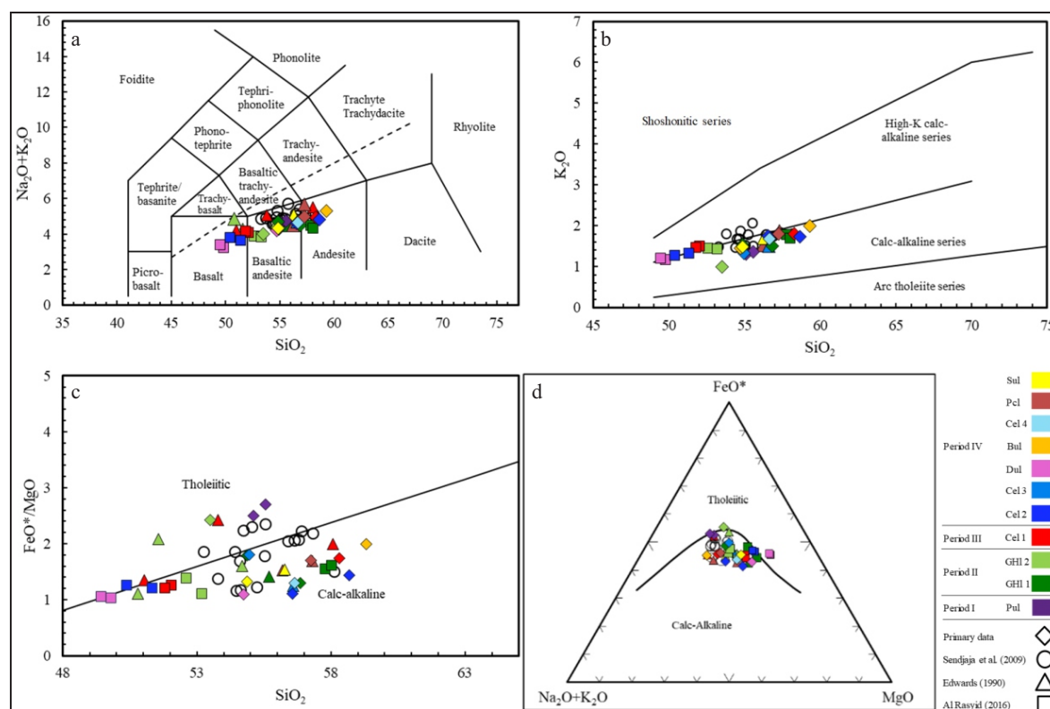
Figure 5. Classifications of magma chemical composition based on its (a) total alkali-silica (TAS; Le Bas et al. , 1986) and magmatic affinity based on (b) \text{K}_2\text{O} vs. \text{SiO}_2 (modified from Peccerillo and Taylor, 1976), (c) \text{FeO}^*/\text{MgO} vs. \text{SiO}_2 (Miyashiro, 1975), and (d) AFM Diagram (Irvine and Baragar, 1971).
