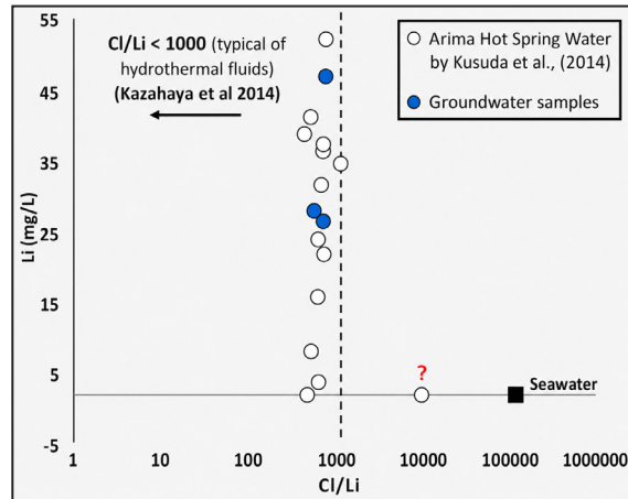
Figure 5. Relationship between Li concentration and Cl/Li ratios for groundwater samples (Umam et al. , 2022) and Arima hot spring waters (Kusuda et al. , 2014) compared with seawater (Oi et al. , 1996). The dashed line (Cl/Li = 1,000) is used as a reference boundary for comparing variations in Cl/Li ratios among the datasets. The four Arima samples previously reported by Umam et al. (2022) plot in the low Cl/Li (<1000) and high Li concentration field while several literature samples show higher Cl/Li values, indicating variability in fluid processes and possible mixing or geochemical modification.
