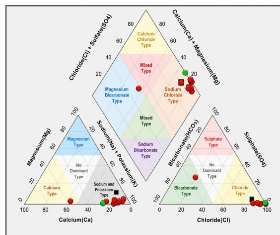
Figure 8. Piper diagram integrated with Li concentration and Cl/Li-based hydrochemical classification for Arima hot spring waters. Red circles represent thermal water, while green circles indicate mixing water, based on Li and Cl concentrations and Cl/Li relationships. Most samples cluster within the Na-Cl type field, while mixing water samples show slight deviations, reflecting dilution and interaction with shallow groundwater. This integrated approach suggests that similar hydrochemical facies may represent different fluid characteristics when Li concentrations and Cl/Li relationships are considered together with major-element compositions.
