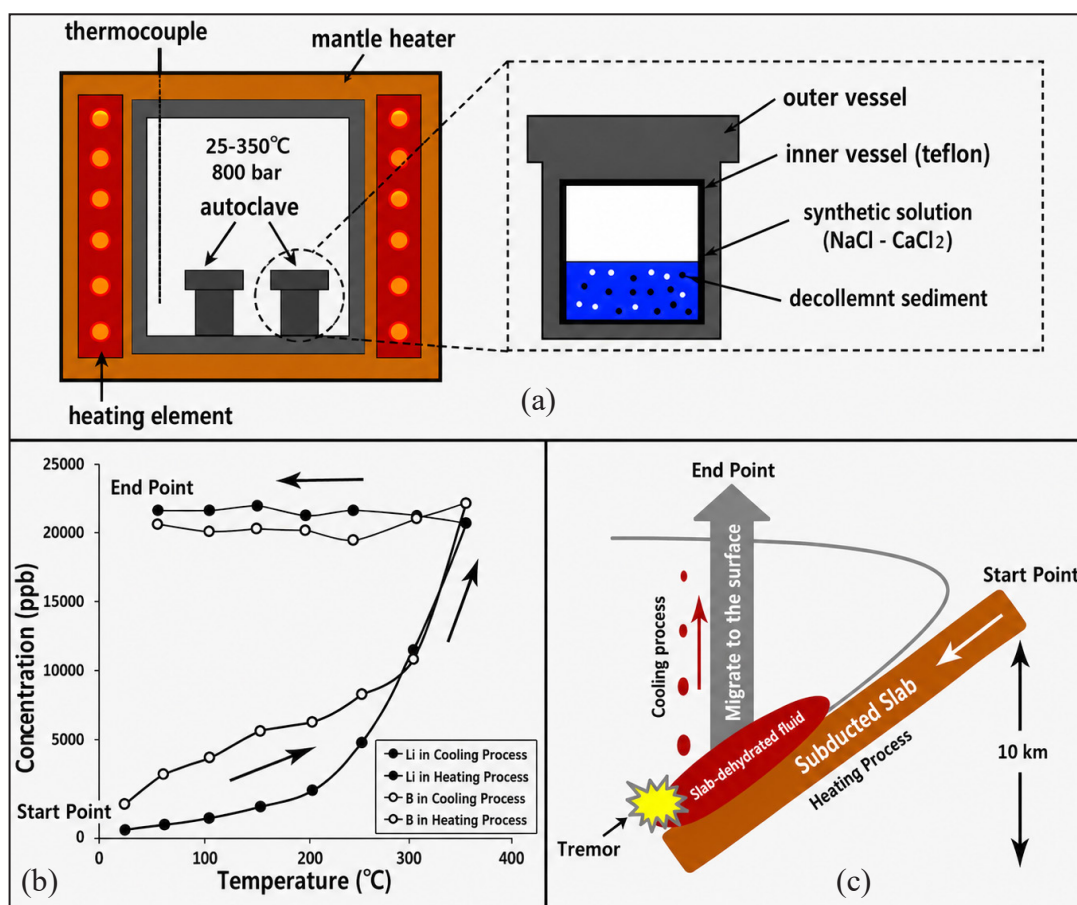
Figure 4. a). Experimental setup for simulating fluid-rock interaction under hydrothermal conditions (25-350°C, 800 bar) using an autoclave system with synthetic saline solution and sediment (You et al. , 1996); b). Temperature-dependent behaviour of Li and B during heating and cooling processes, highlighting the sensitivity of Li to thermal conditions and fluid evolution; c). A conceptual model linking slab dehydration processes to fluid migration, illustrating the generation of slab-derived fluids and their ascent toward the surface.
