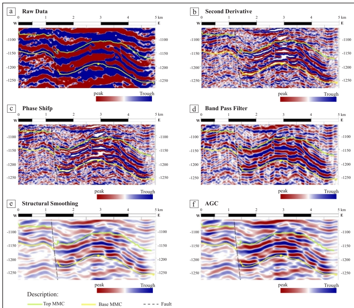
Figure 4. a) Raw data seismic, b) Attribute Second Derivative, c) Phase Shift, d) Band Pass Filter, e) Structural Smoothing, f) AGC. (Green horizon shows top of MMC formation).
