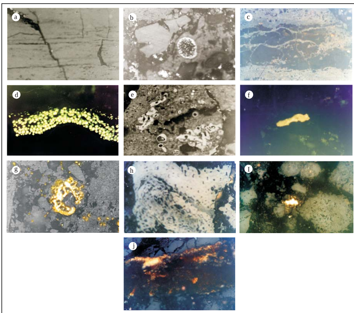
Figure 9. Photomicrographs of macerals and mineral matter:
