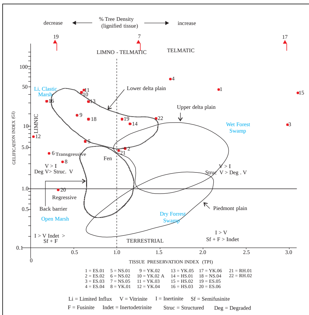
Figure 11. Coal facies diagram of TPI versus GI (Diesel 1965, 1986 ; Kalkreuth et al., 1989) of coals studied that displays their paleodepositional environment.
