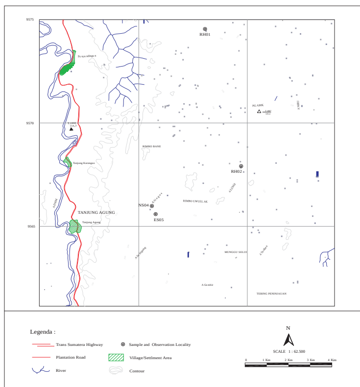
Figure 7. Outcrop sample and observation locality map of South Banko area.
