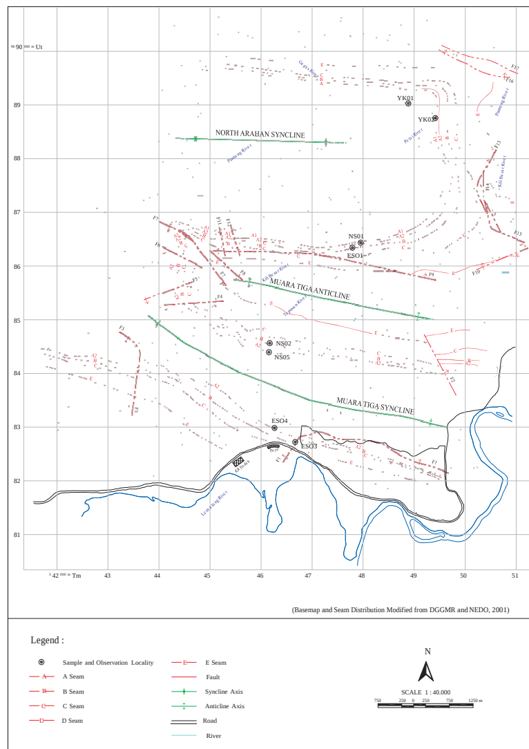
Figure 4. Outcrop sample and observation locality map of North and South Arahan areas.
