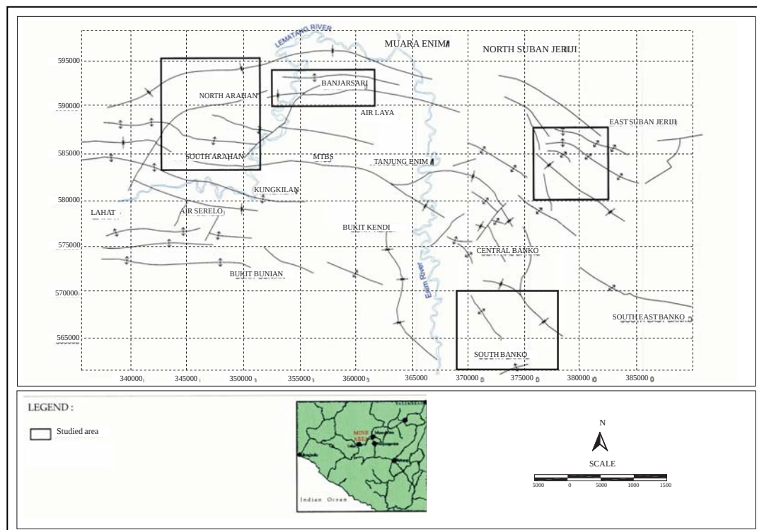
Figure 1. Locality map of the studied areas situated in the PTBA coal field, South Sumatra.
