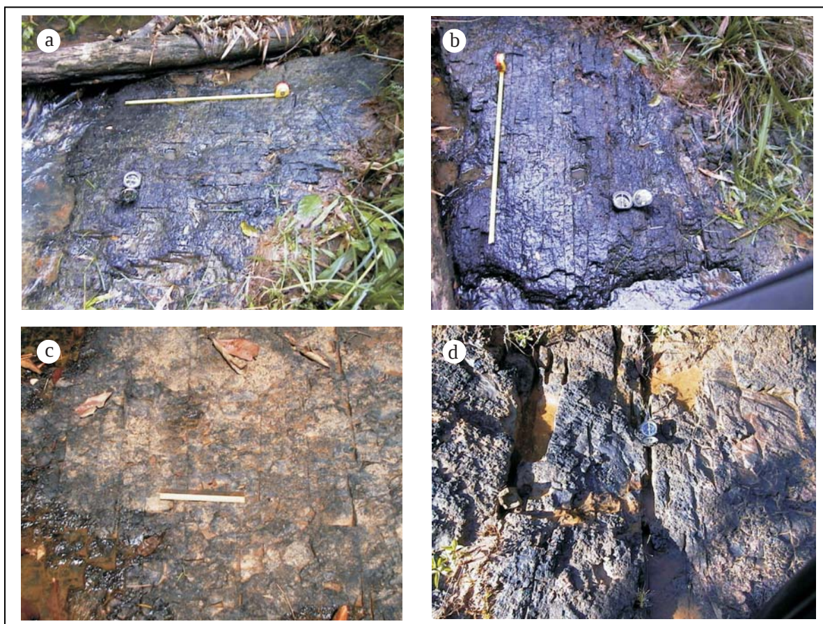
Figure 8. Photographs of coal outcrops in studied area:
