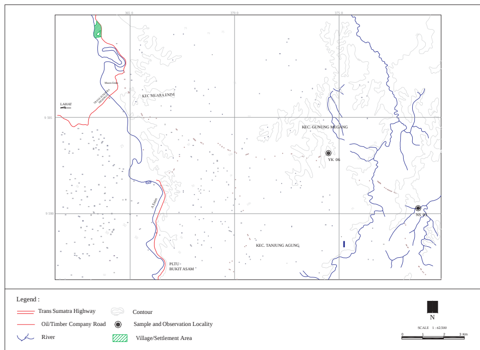
Figure 6. Outcrop sample and observation locality map of the Subanjeriji area.
