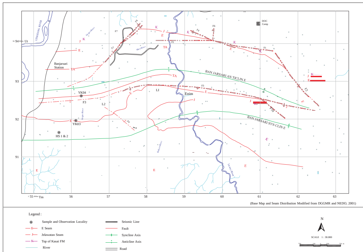
Figure 5. Outcrop sample and observation locality map of the Banjarsari area.
