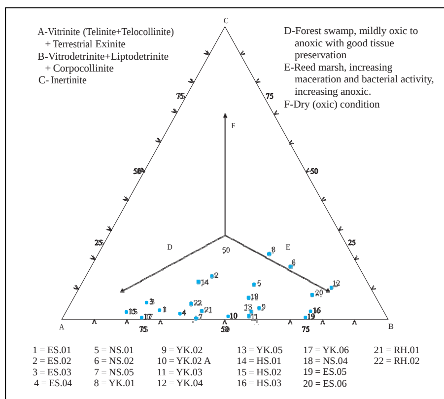
Figure 10. Ternary facies diagram of coals studied showing their paleodepositional facies (based on Singh et al. 's. diagram, 2010).
