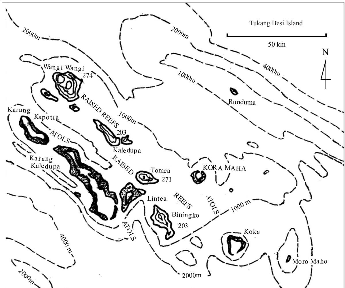
Figure 6. Reef caps, atolls, and submarine relief of the Tukang Besi.
