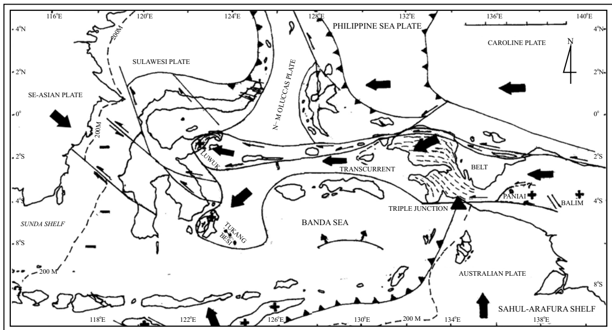
Figure 2. Plate-triple junction and transcurrent belt in East Indonesia (Katili, 1980).
