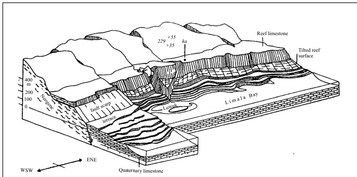
Figure 5. Block diagram of the raised reefs near Luwuk, East Sulawesi (Sumosusastro et al. , 1999).
