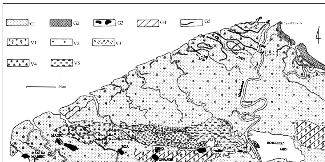
Figure 3. Mamberamo Delta, affected by sinistral transcurrent faulting. G1: alluvium, G2: beach ridges, G3: mud volcanoes, G4: hills unspecified, G5: depth of crystalline basement, V1: hill forest, V2: swamp forest, V3: low swamp vegetation, V4: mangrove, and V5: grass/rush marsh.
