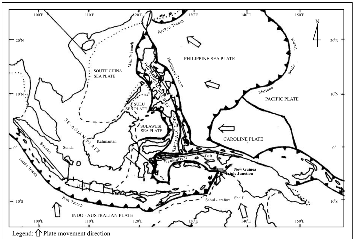
Figure 1. The plate-tectonic configuration of Indonesia and surroundings (Katili, 1980).
