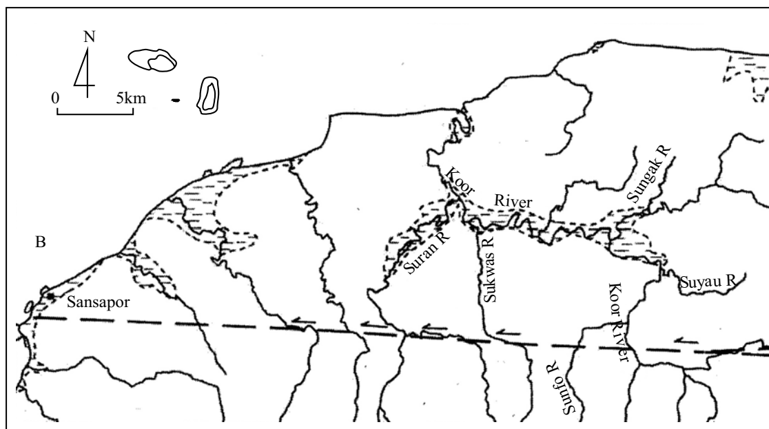
Figure 4. River offsets along the sinistral transcurrent Koor Fault, "bird's head".
