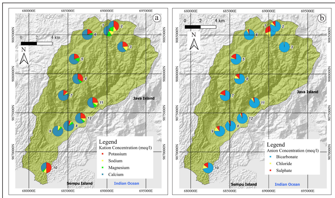
Figure 7. (a). Cation and (b). anion in groundwater of Penguluran Basin.
