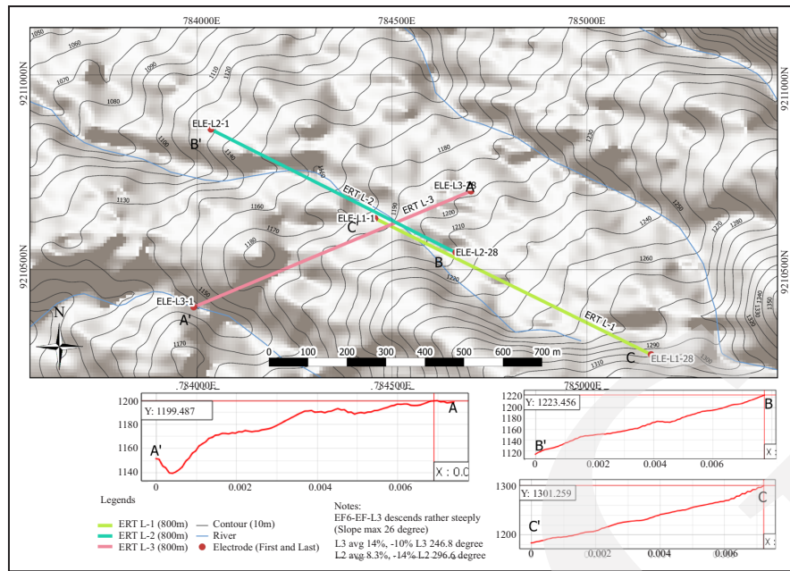
Figure 4. The map depicts the location and orientation of the Electrical Resistivity Tomography lines in the studied area (top). The elevation profiles of each ERT line (A'-A, B'-B, C'-C) include the placement of electrical electrodes (bottom).
