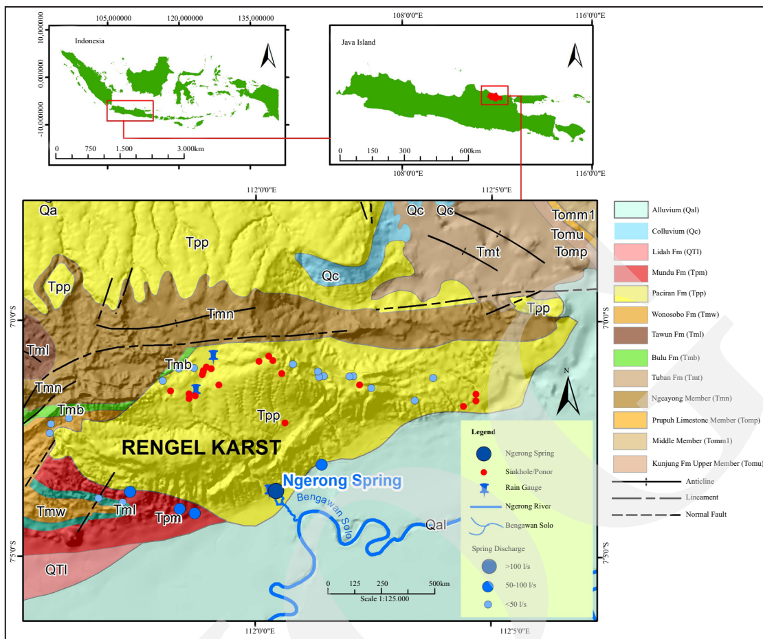
Figure 1. Recharge area of The Ngerong Spring system in Rengel Karst, East Java
