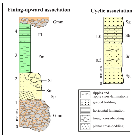
Figure 8. A facies model of the Citalang Formation (Setiadi, 1998).
