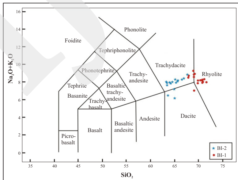
Figure 6. SiO 2 vs Na 2 O+K 2 O classification diagram for BI-1 and BI-2 showing the compositions of dacite to rhyolite. Field from Le Maitre (1989).
