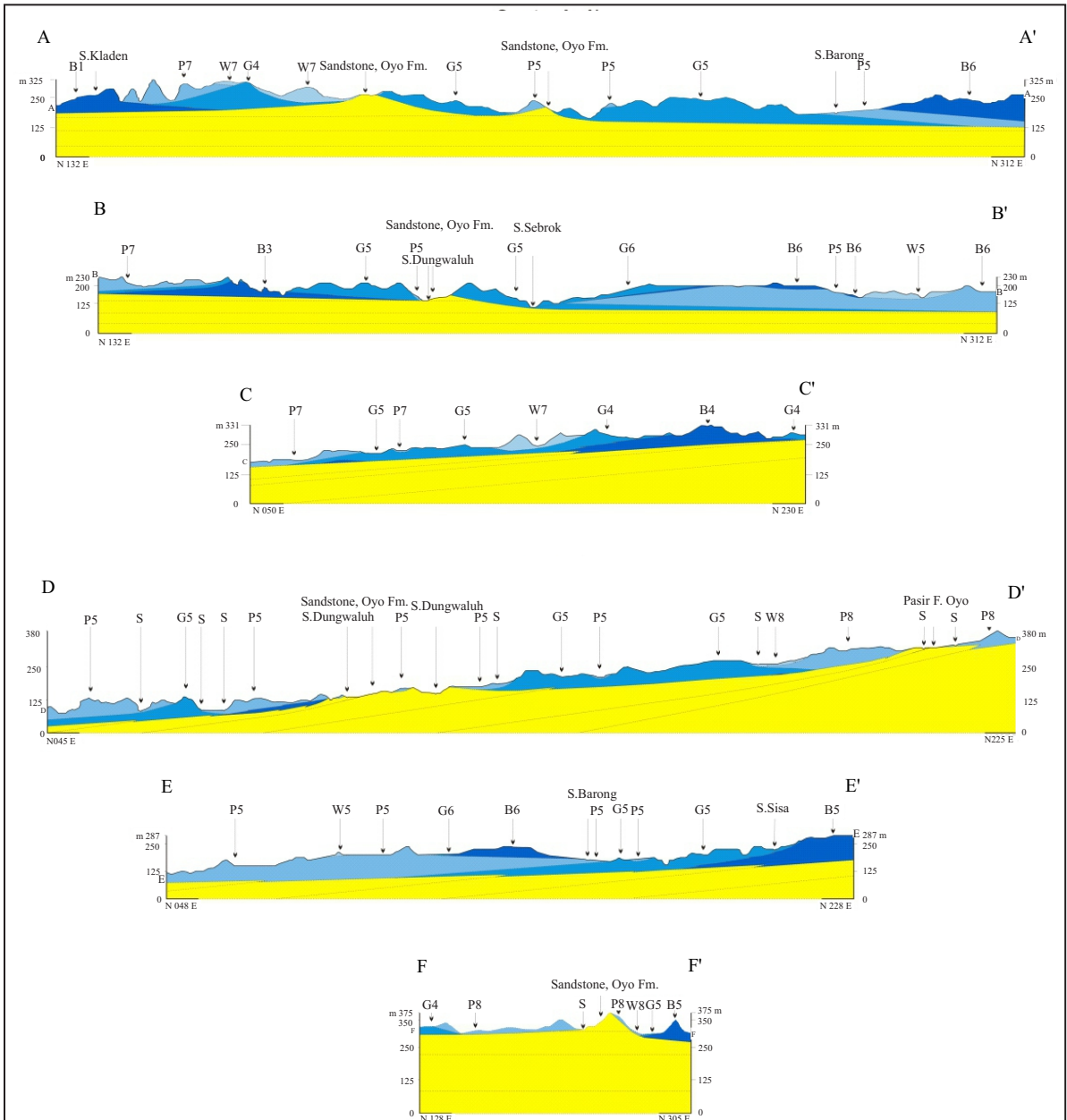
Figure 7. The lithofacies sections of Punung Fm. shows an almost similar gentle dipping to Jaten Formation (the paleoreef base) and one reef unit overlaid to each other. It indicates the fringing reef (based on geological map in Figure 6/Jaran Cave).
