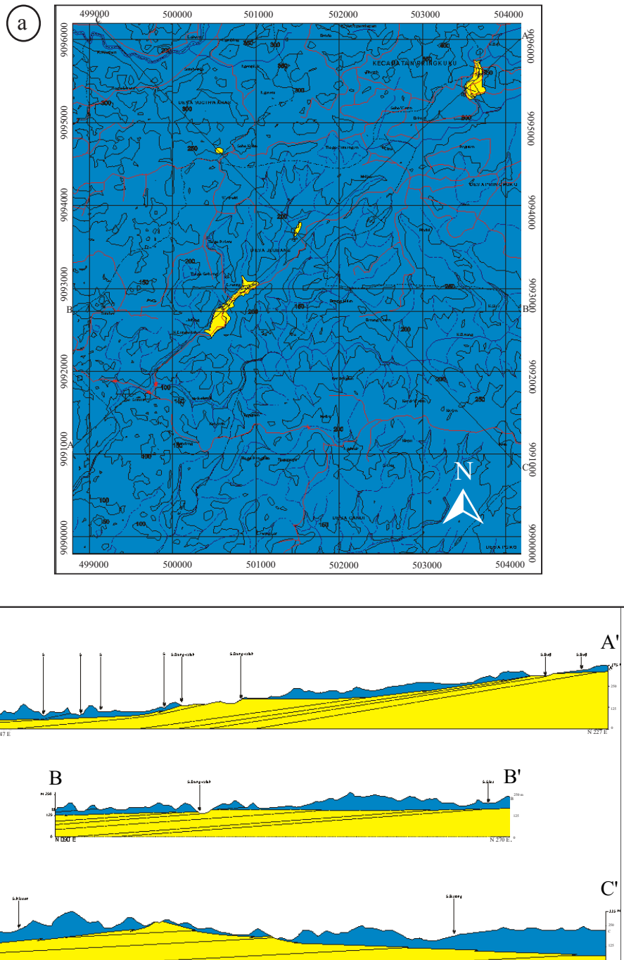
Figure 4. a) Geologic map of Jlungang area. The Jaten Formation (Yellow color) distributed spottly and NE orientations. Almost 90% outcropped of paleoreef Punung Formation (Blue color). Black crosslines is direct of sections (see below), b) The geologic sections of Jaten and Punung Formation conical hills and karst topography, gentle dipping to the south.
