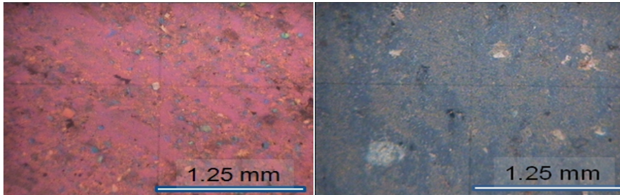
Figure 5. Thin sections of wacky quartz sandstone of Jaten Formation showing muddy dominantly. Right: crossnicol; Left: parallel nicol.
