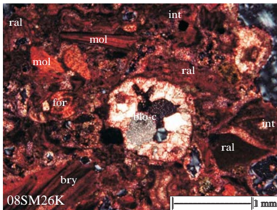
Figure 11. Photomicrograph of bioclastic packstone displaying several mollusks (mol), foraminifera (for), bryozoans (bry), intraclasts (int), and bioturbation pores infilled by blocky drussy mosaic anhedral cement (blo-c) from meteoric phreatic environment. Sample SM26K, with cross nicol and without carbonate staining.
