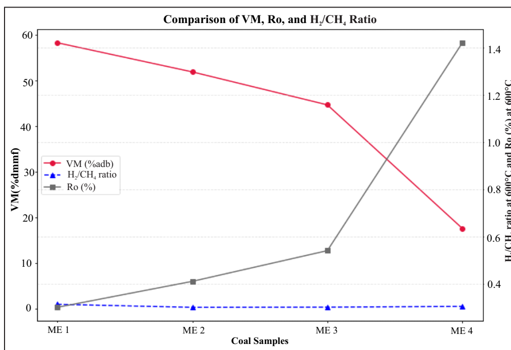
Figure 5. Comparison of Volatile Matter (VM), Vitritine Reflectance (Ro), and H 2 /CH 4 ratio.
