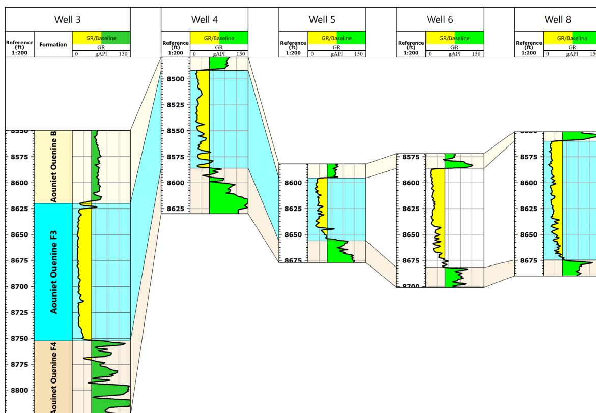
Figure 2. F3 Sandstone (Aouinet Uennin Formation) boundary delineation by gamma ray logs of the studied wells, Al Wafa oil field - Ghadamess Basin, Libya.
