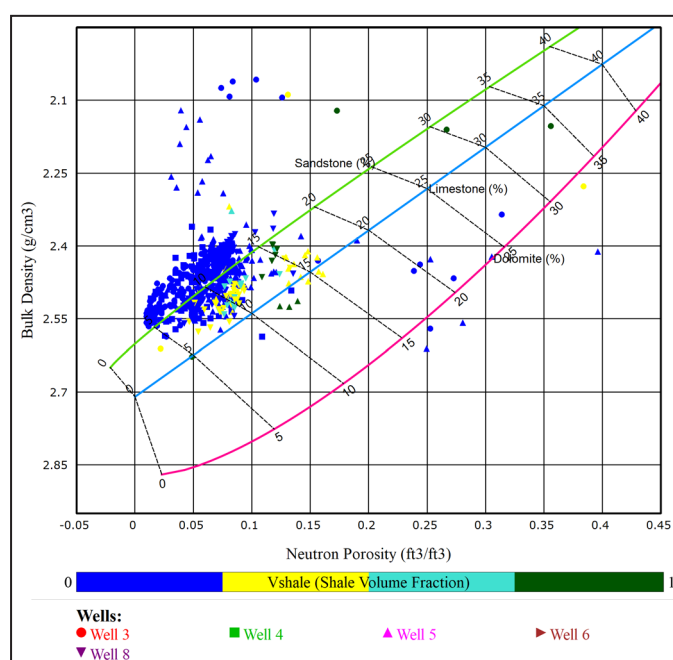
Figure 3. Bulk density versus neutron porosity between the studied wells, F3 Sandstone reservoir (Aouniet-Ouenine Formation).
