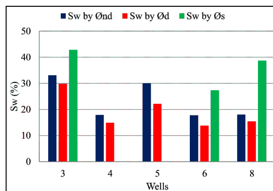
Figure 7. Comparison of the average water saturation estimation by using different porosity logs.
