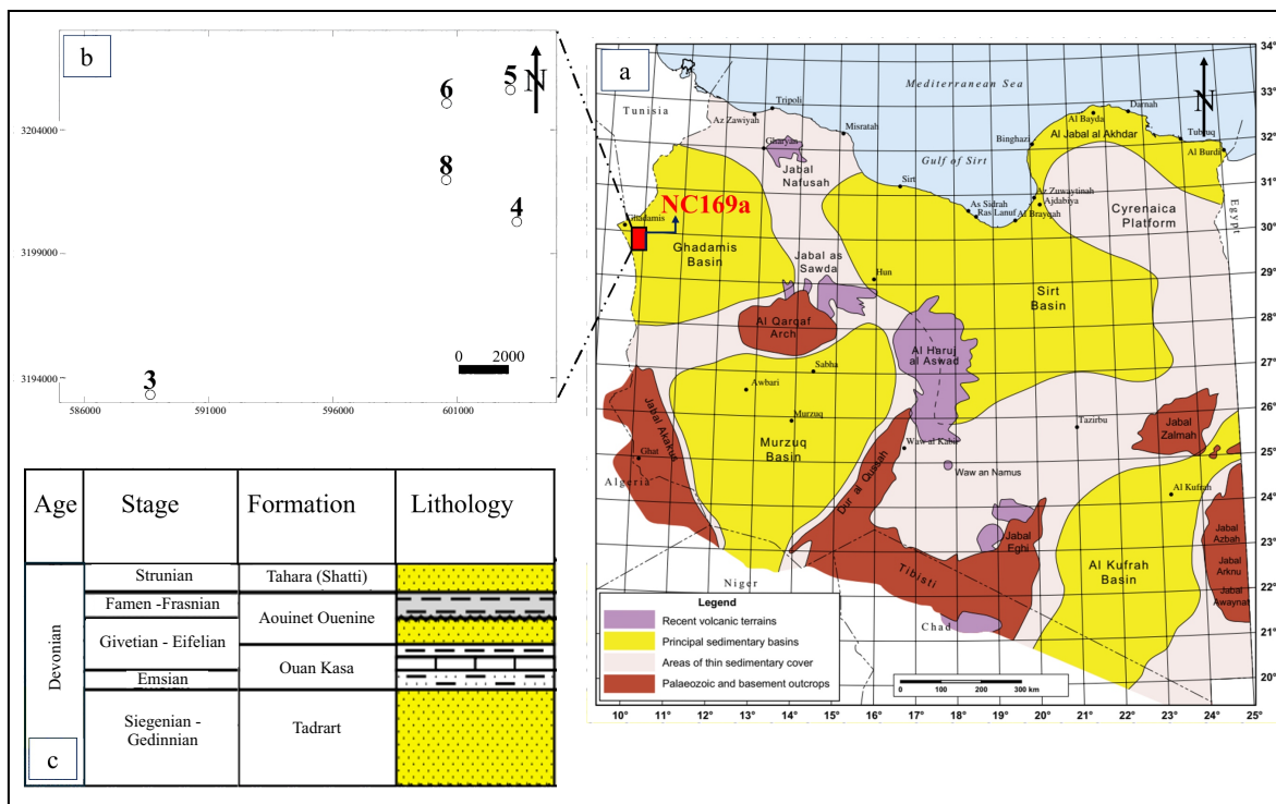
Figure 1. a. Major sedimentary basins of Libya (after Hallett and Clark-Lowes, 2016), b. Location of the studied wells from Al Wafa Field-NC 169a, and c. Sequence stratigraphy of the Devonian age (after Hallett and Clark-Lowes, 2016).
