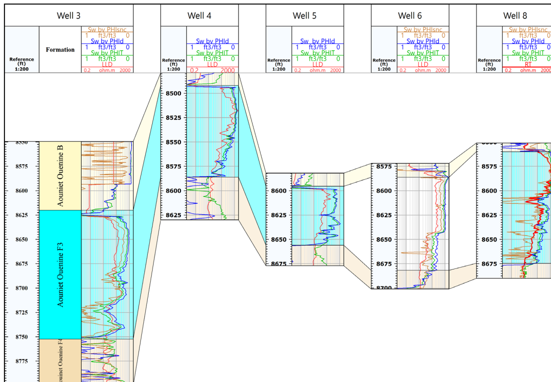
Figure 6. Comparison between the water saturation ( S_w ) that has resulted in different log porosity of each studied well and the deep resistivity ( R_d ) logs of the F3 Sandstone reservoir (Aouniet-Ouenine Formation).
