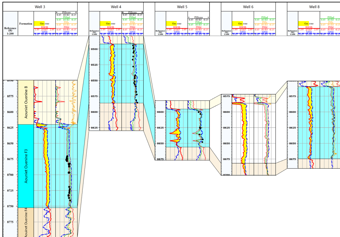
Figure 5. Gas detection zone by the neutron porosity ( \Phi_n ) and bulk density ( \rho_b ) a correlation among the studied wells of the F3 Sandstone reservoir (Aouniet-Ouenine Formation).
