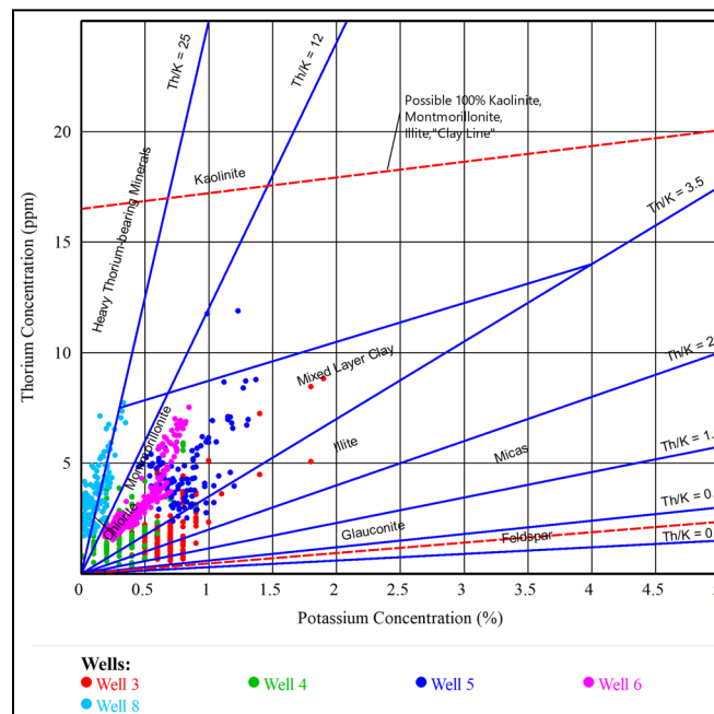
Figure 4. Thorium (Th) and potassium (K) concentration cross plot of the studied wells, F3 Sandstone reservoir (Aouniet-Ouenine Formation).
