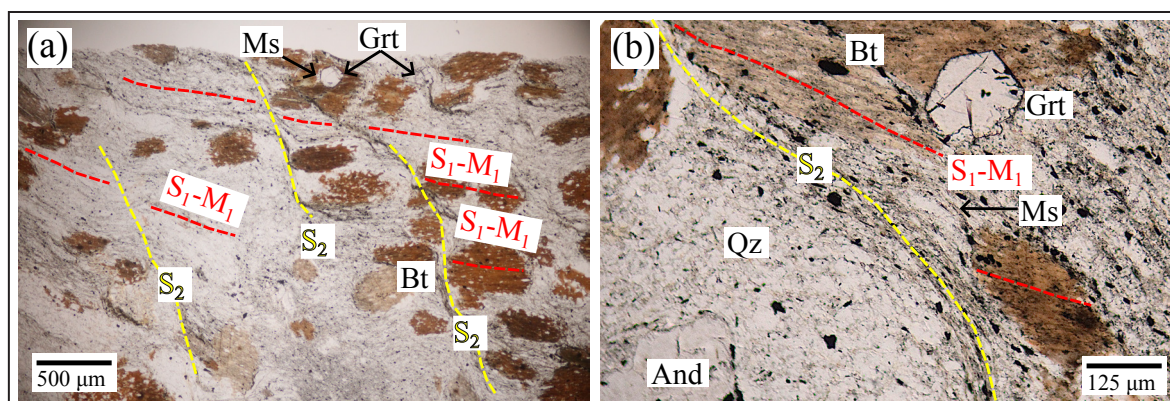
Figure 4. Microstructural features of garnet-andalusite-biotite schist (sample 12T01O). (a) S_1 foliation is defined by aligned muscovite, with biotite and fine-grained garnet occurring parallel to foliation; S_2 crenulation locally overprints S_1 . (b) Close-up showing S_2 crenulation cleavage affecting quartz, muscovite, biotite, and andalusite, locally deflecting the earlier S_1 foliation.
