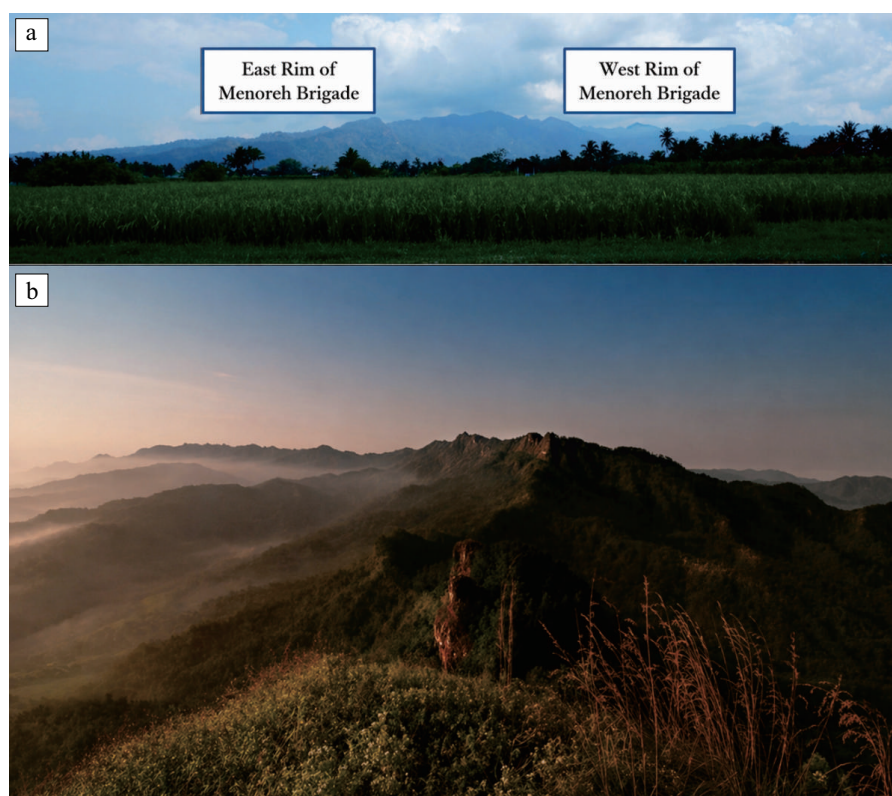
Figure 7. The Appearance of the steep escarpment on the west - east side of Menoreh Brigade, photo taken from the north of the Menoreh Mountains (a); The curved structure opens to the north of Menoreh Brigade taken from the summit on the west side (b) ( https://www.flickr.com/photos/hanafichi/14324789537 ).
