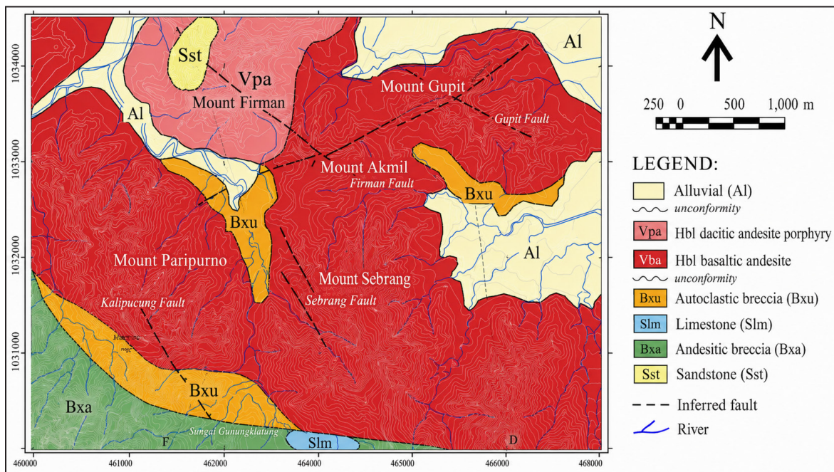
Figure 10. Geological map of Gunung Gupit and its vicinity (Idrus et al. , 2024).
