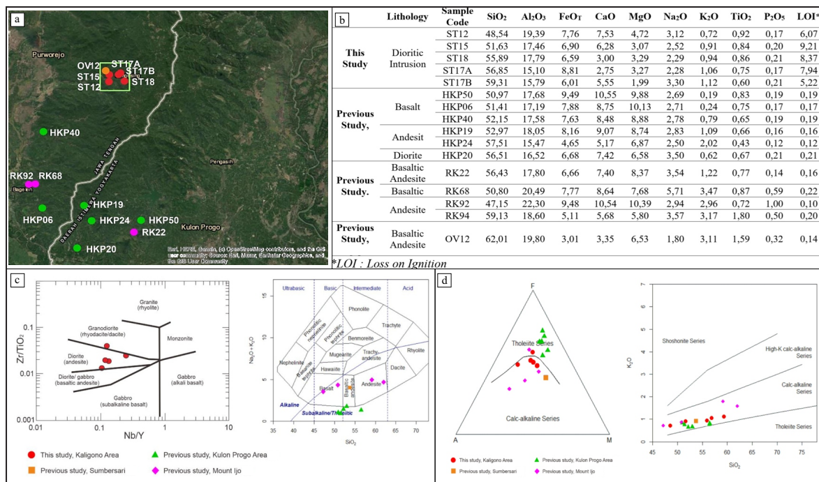
Figure 11. Geochemical data taken from the research by Astuti et al. (2024) with an explanation; (a) Sampling location and previous studies in Summersari (orange circle), Kulon Progo area (green circles), and Mount Ijo (purple circles); (b) Major oxides abundance (%) in several igneous rock samples; (c) Zr/TiO 2 vs. Nb/Y of Kaligono samples and Silica versus total alkali; (d) AFM ternary diagram and the SiO 2 vs. K 2 O diagram where data is taken at the location at Ijo Brigade, Gajah Brigade and its surroundings.
