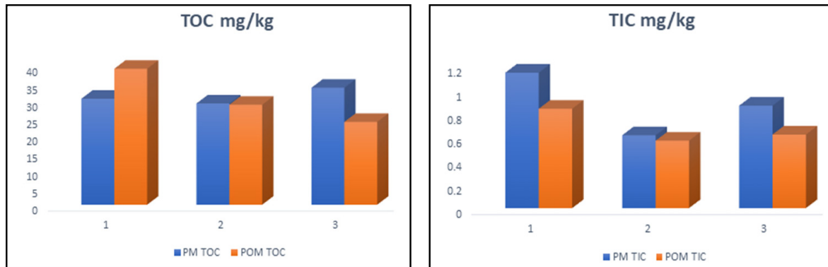
Figure 3. Concentrations of a) Total Organic Carbon (TOC mg/kg) and b) Total Inorganic Carbon (TIC mg/kg) in surface sediment samples in the PL during the PM and PoM seasons.
