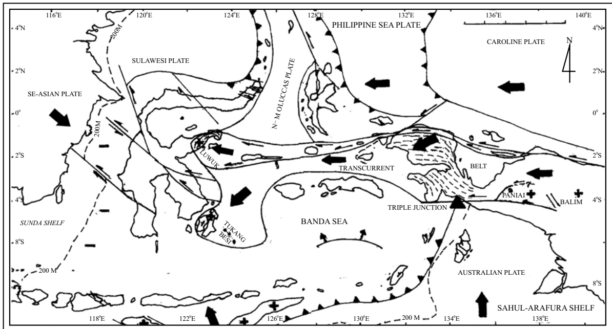
Figure 2. Plate-tuple junction and transcurrent belt in East Indonesia (Katili, 1980).
