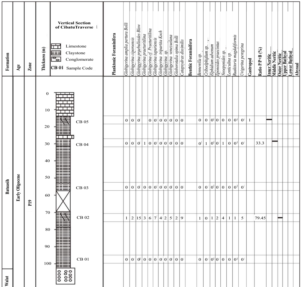
Figure 7. Foraminifera distribution in the Cibatú traverse.
