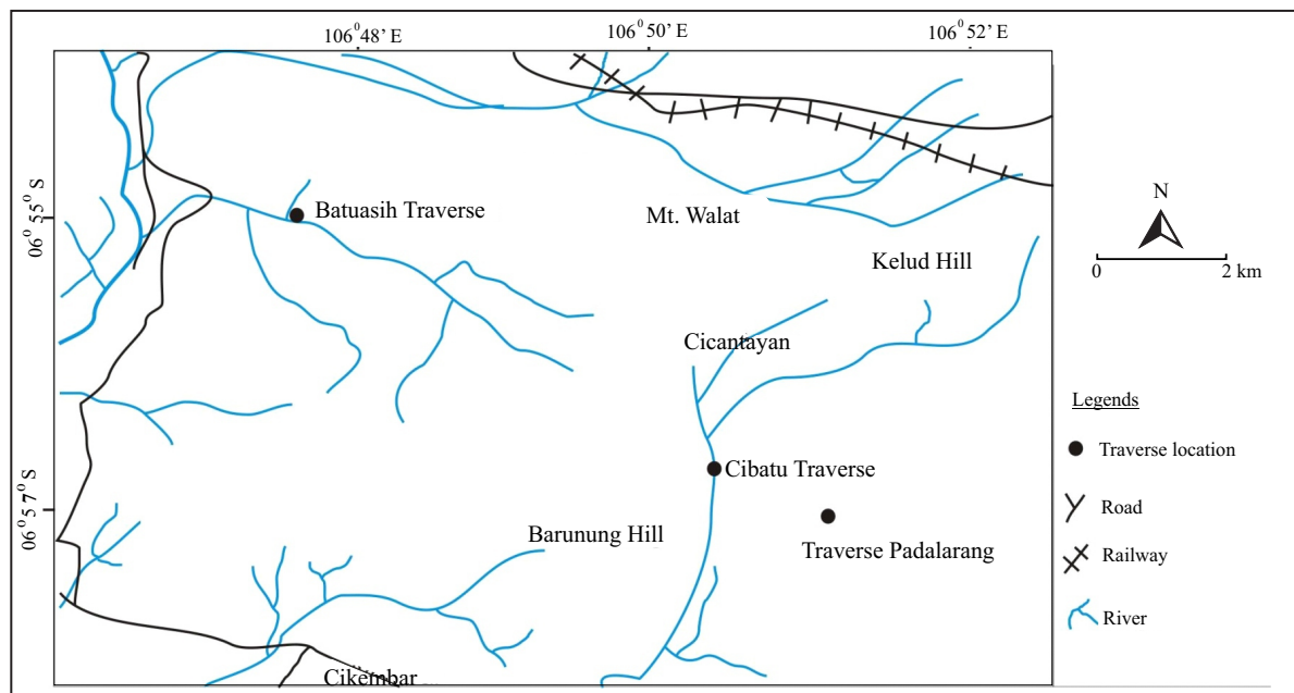
Figure 2. Locality map of outcrop studied of the Batuasih Formation, Sukabumi.
