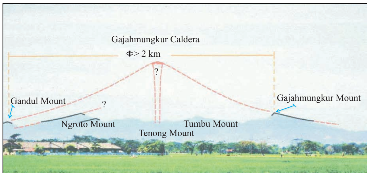
Figure 2. The reconstruction of Gunung Gajahmungkur proper shows the ancient Gajahmungkur Volcano. Three remnants of calderas are observable, namely Gajahmungkur-Gandul Caldera (the largest), unnamed caldera, and Ngroto Caldera. In the central part the basaltic andesite domes namely Tenong Hill and Tumbu Hill are also observable. These domes developed in the Gajahmungkur Caldera (somma) indicating the terminating stage of the ancient Gajahmungkur Volcano. The crater is about two kilometers across (Hartono, 2010). The photograph was taken from NW of Gajahmungkur by H. G. Hartono.
