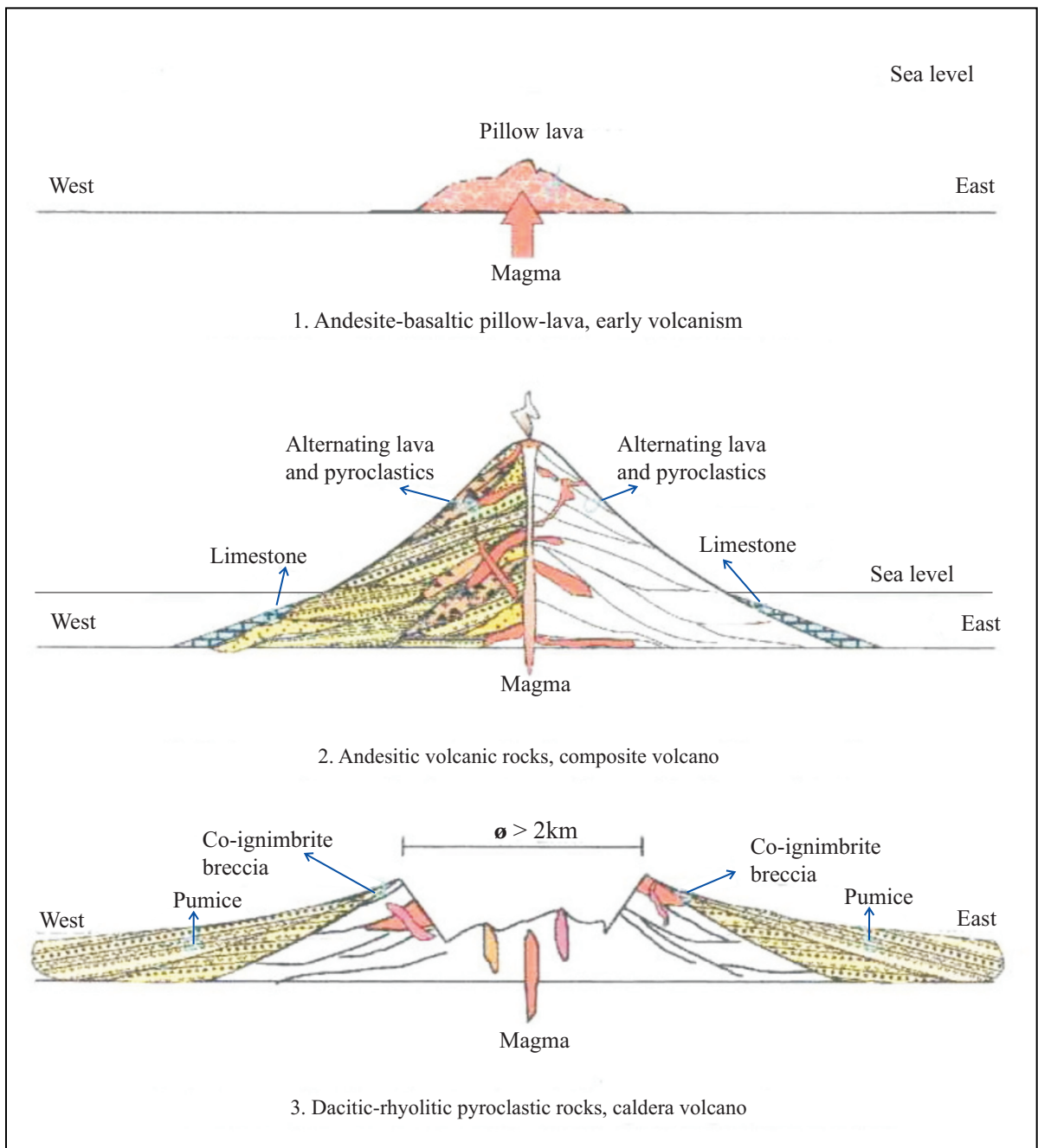
Figure. 3. The illustration shows the development of Gajahmungkur Volcano starting with the formation of lava flows with pillow structure indicating subaqueous deposition (above), followed by the formation of a composite strato volcano island (middle), and finally the self destruction resulting in the formation of caldera (below).
